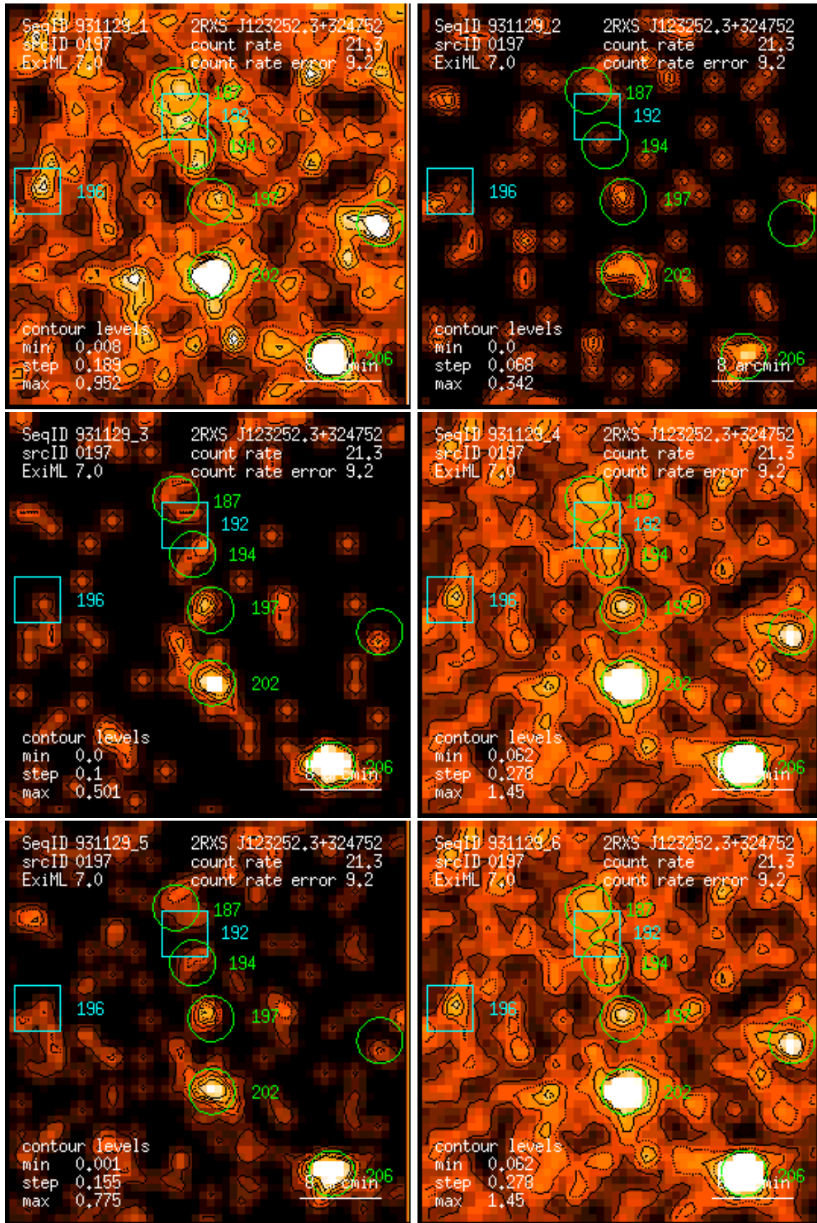
Figure 197: RASS 931129: detection 0197: band rate images, Gaussian filter: (1) PSPC channels 11 – 41, (2) 52 – 90, (3) 91 – 201, (4) 11 – 235, (5) 52 – 201, (6) 11 – 201. Broad band rates in counts/ks. Band rate contour levels in counts/ks/arcmin 2 .
