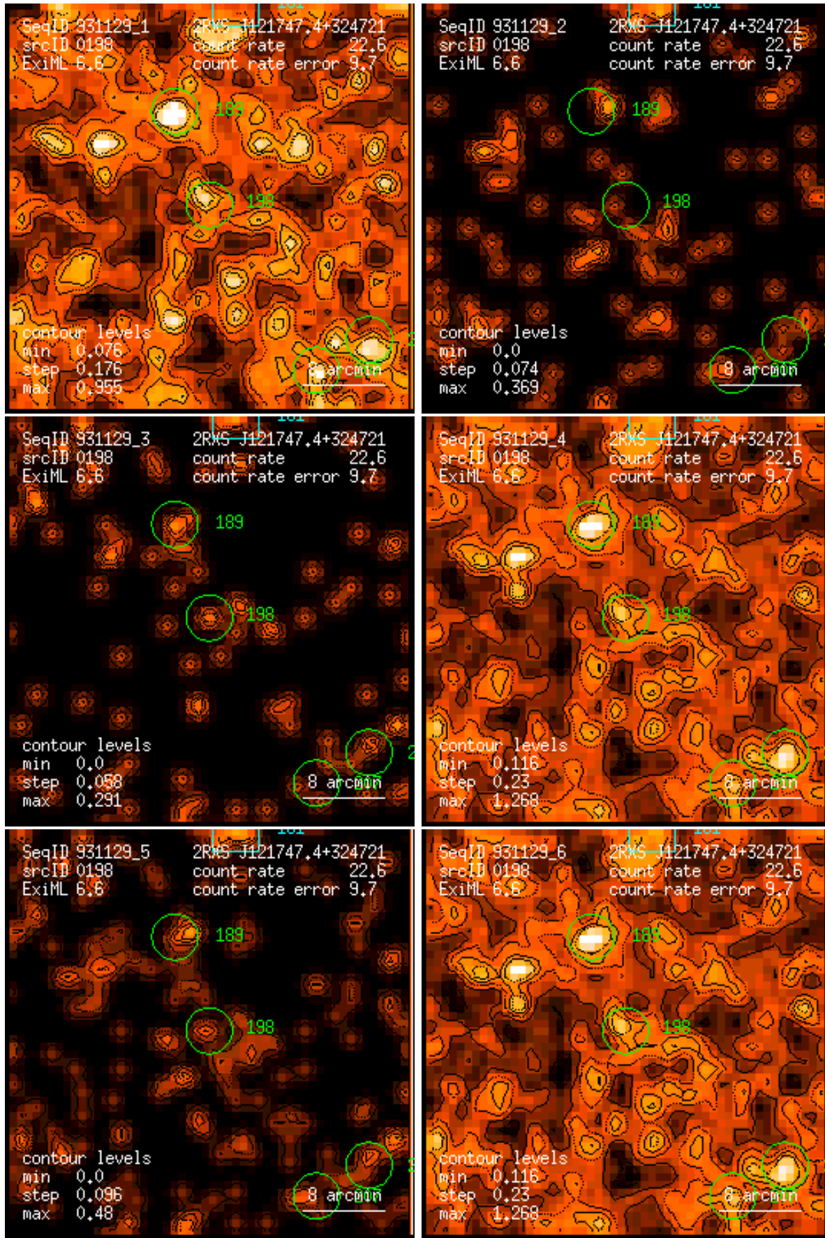
Figure 198: RASS 931129: detection 0198: band rate images, Gaussian filter: (1) PSPC channels 11 – 41, (2) 52 – 90, (3) 91 – 201, (4) 11 – 235, (5) 52 – 201, (6) 11 – 201. Broad band rates in counts/ks. Band rate contour levels in counts/ks/arcmin 2 .
