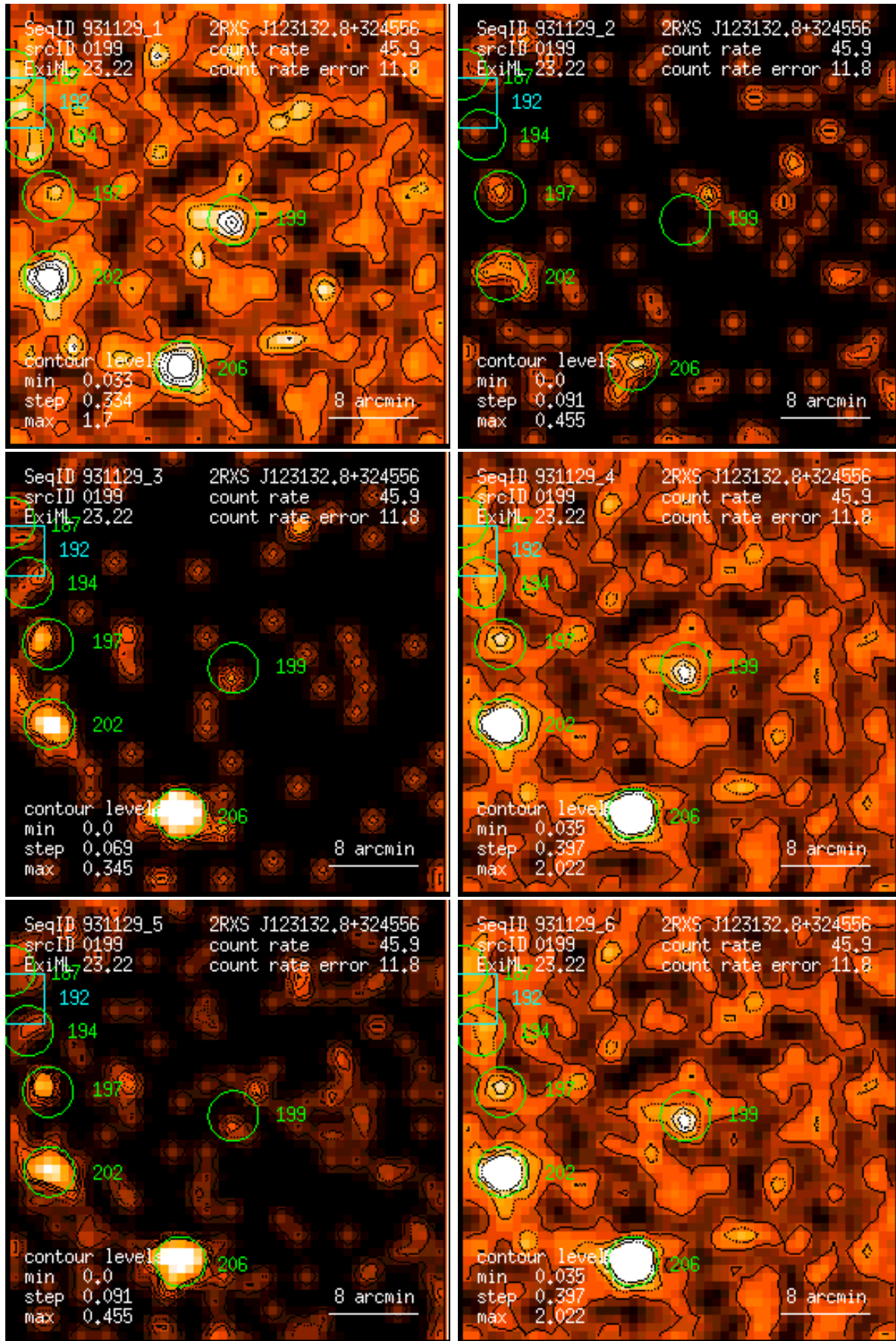
Figure 199: RASS 931129: detection 0199: band rate images, Gaussian filter: (1) PSPC channels 11 – 41, (2) 52 – 90, (3) 91 – 201, (4) 11 – 235, (5) 52 – 201, (6) 11 – 201. Broad band rates in counts/ks. Band rate contour levels in counts/ks/arcmin 2 .
