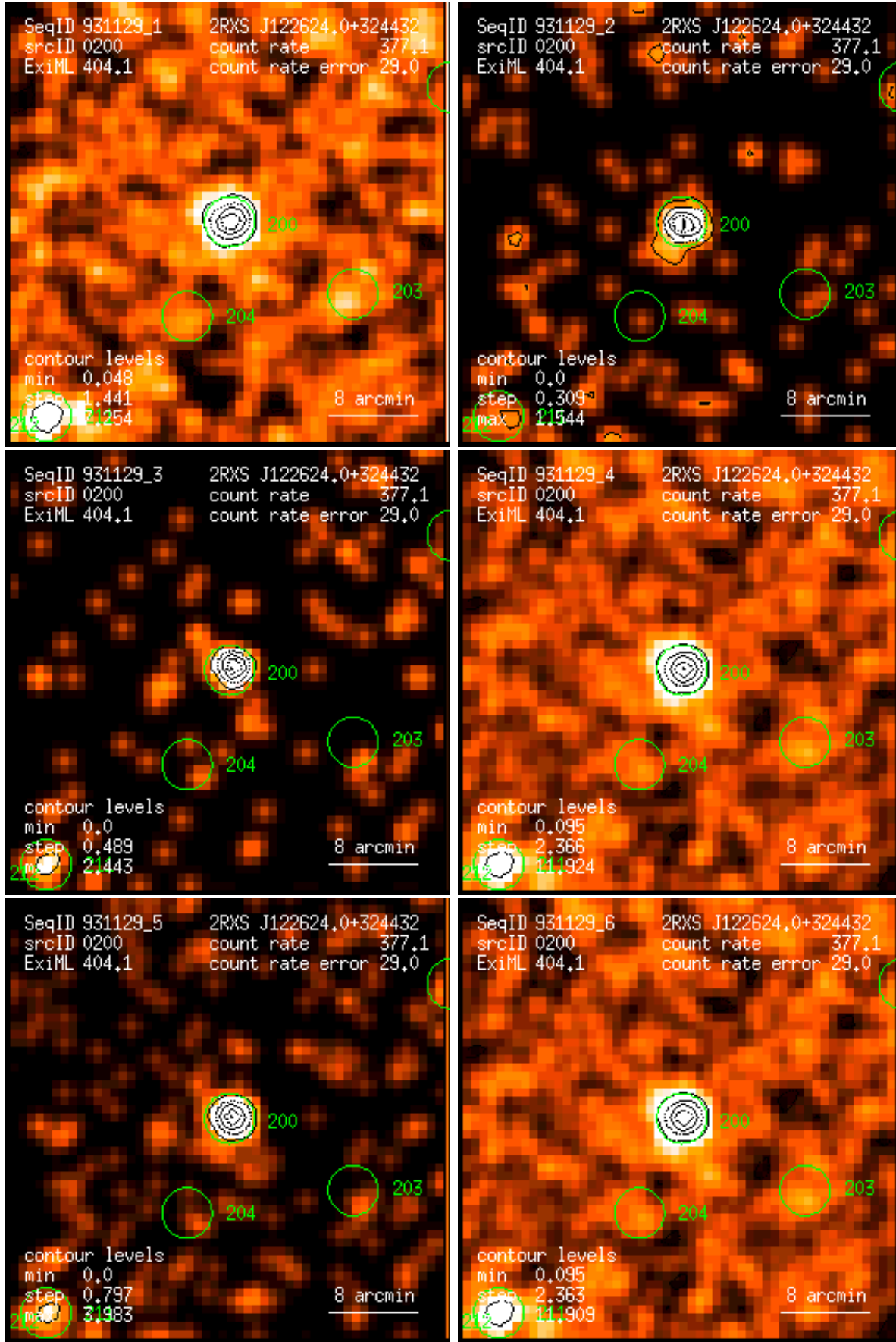
Figure 200: RASS 931129: detection 0200: band rate images, Gaussian filter: (1) PSPC channels 11 – 41, (2) 52 – 90, (3) 91 – 201, (4) 11 – 235, (5) 52 – 201, (6) 11 – 201. Broad band rates in counts/ks. Band rate contour levels in counts/ks/arcmin 2 .
