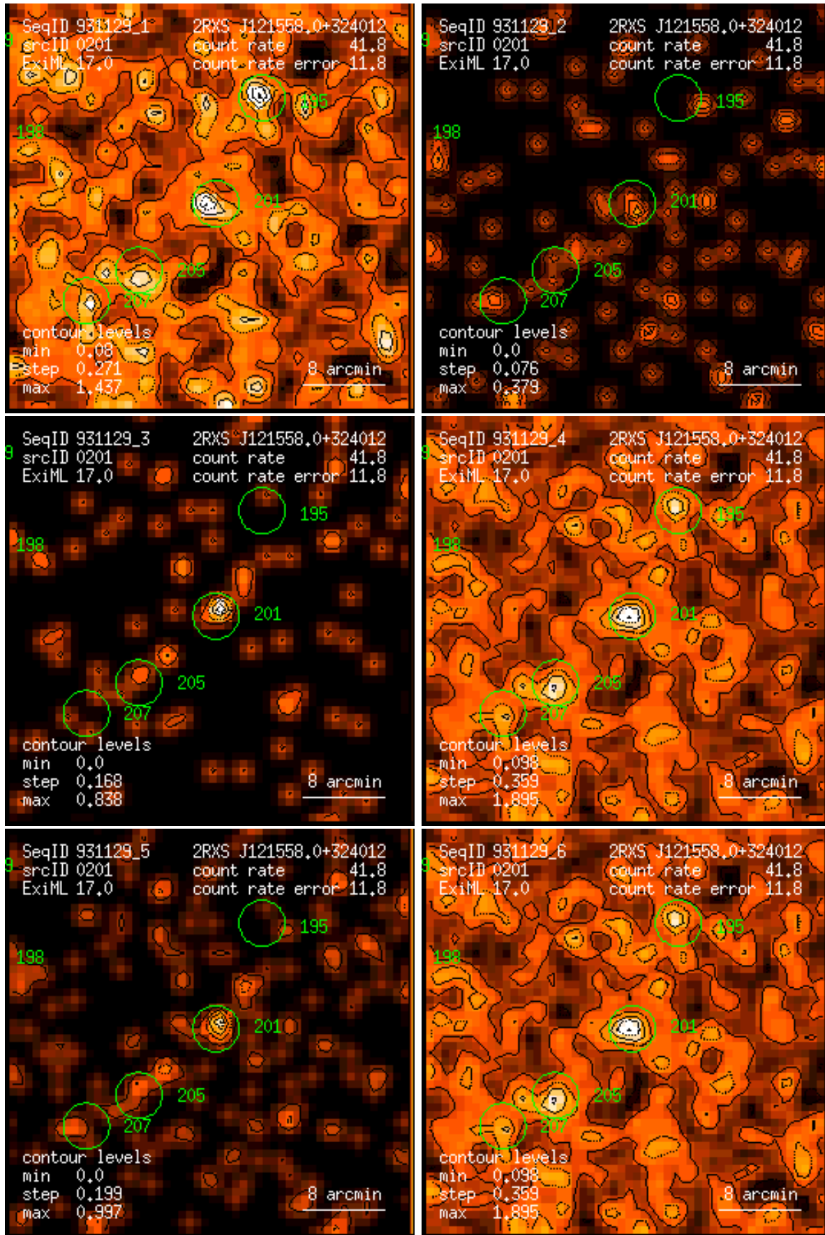
Figure 201: RASS 931129: detection 0201: band rate images, Gaussian filter: (1) PSPC channels 11 – 41, (2) 52 – 90, (3) 91 – 201, (4) 11 – 235, (5) 52 – 201, (6) 11 – 201. Broad band rates in counts/ks. Band rate contour levels in counts/ks/arcmin 2 .
