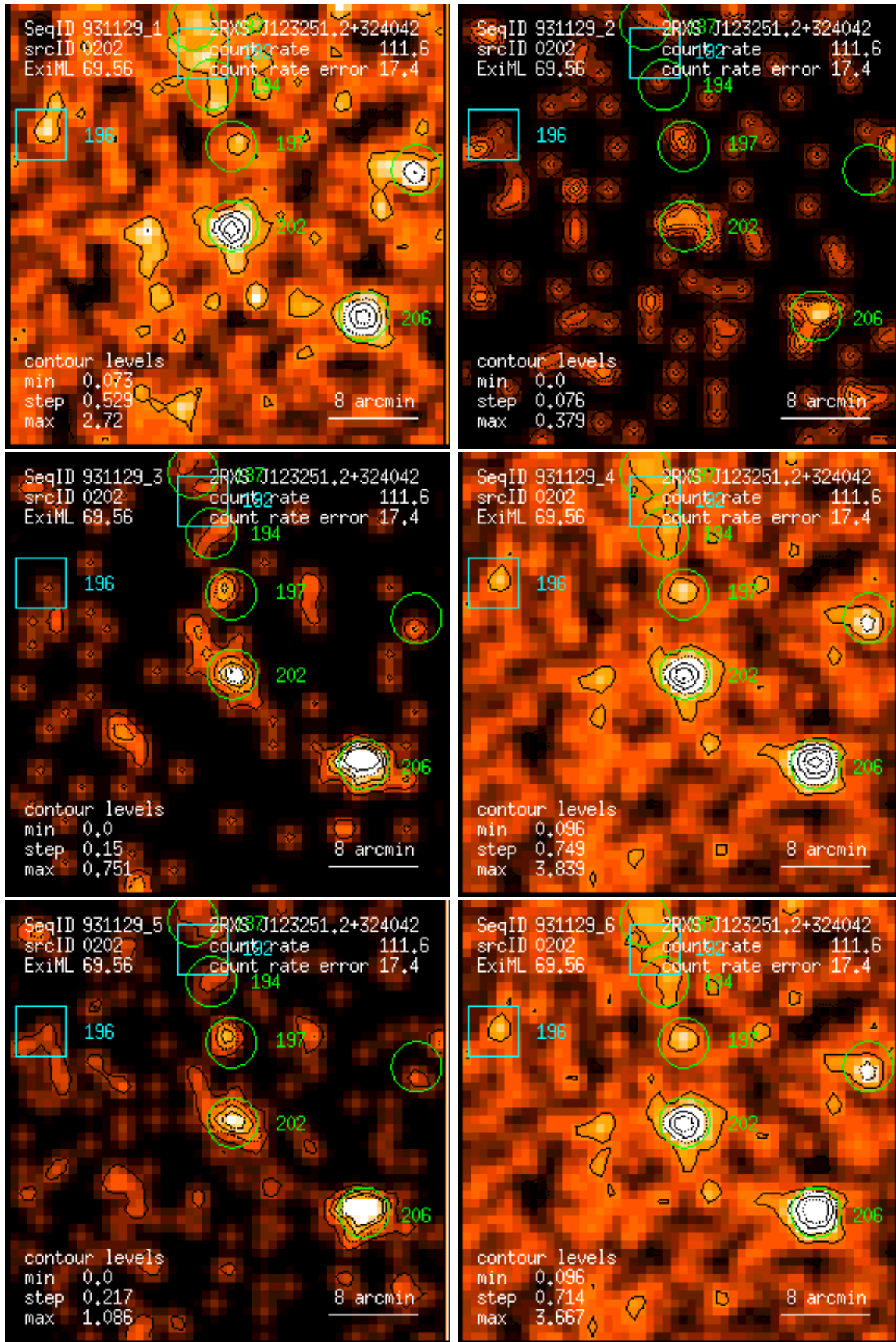
Figure 202: RASS 931129: detection 0202: band rate images, Gaussian filter: (1) PSPC channels 11 – 41, (2) 52 – 90, (3) 91 – 201, (4) 11 – 235, (5) 52 – 201, (6) 11 – 201. Broad band rates in counts/ks. Band rate contour levels in counts/ks/arcmin 2 .
