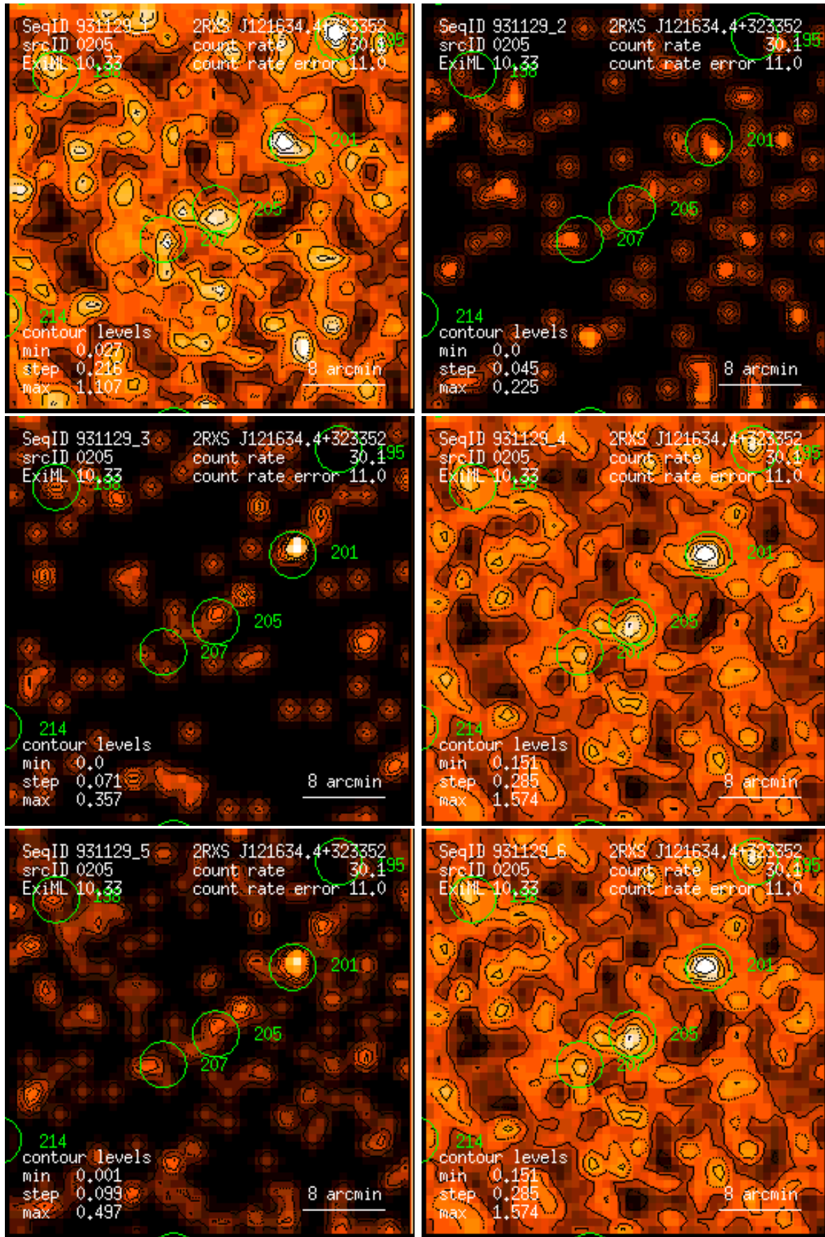
Figure 205: RASS 931129: detection 0205: band rate images, Gaussian filter: (1) PSPC channels 11 – 41, (2) 52 – 90, (3) 91 – 201, (4) 11 – 235, (5) 52 – 201, (6) 11 – 201. Broad band rates in counts/ks. Band rate contour levels in counts/ks/arcmin 2 .
