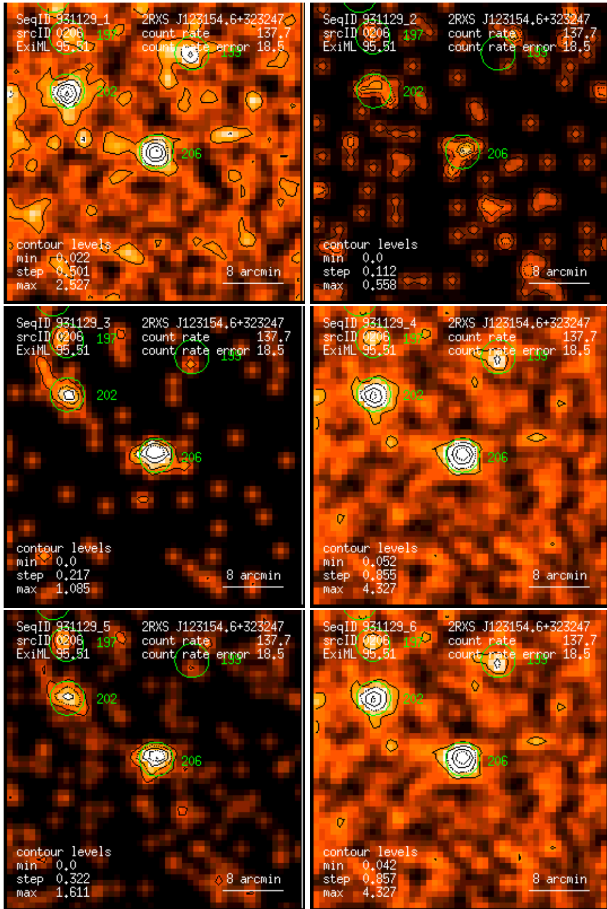
Figure 206: RASS 931129: detection 0206: band rate images, Gaussian filter: (1) PSPC channels 11 – 41, (2) 52 – 90, (3) 91 – 201, (4) 11 – 235, (5) 52 – 201, (6) 11 – 201. Broad band rates in counts/ks. Band rate contour levels in counts/ks/arcmin 2 .
