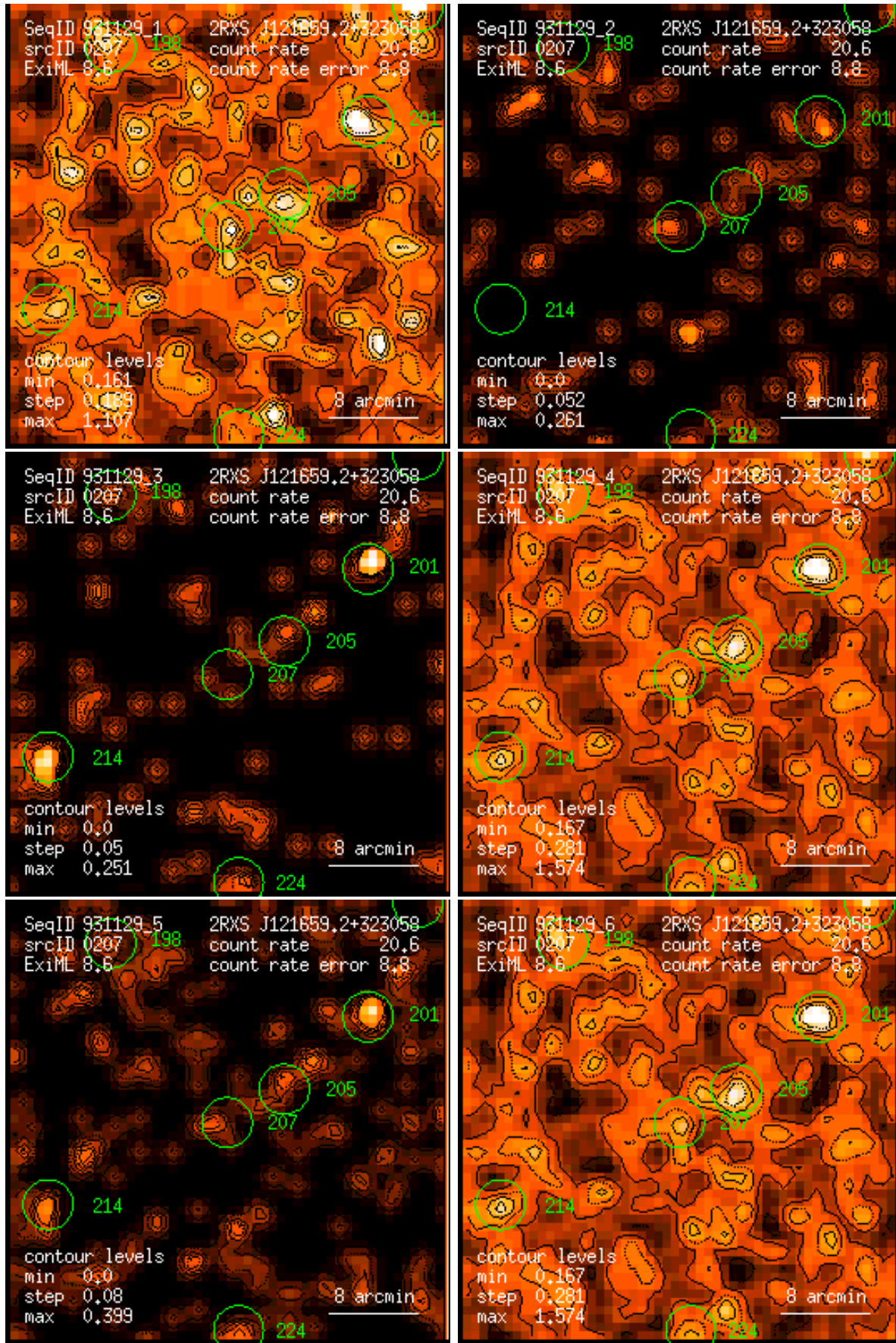
Figure 207: RASS 931129: detection 0207: band rate images, Gaussian filter: (1) PSPC channels 11 – 41, (2) 52 – 90, (3) 91 – 201, (4) 11 – 235, (5) 52 – 201, (6) 11 – 201. Broad band rates in counts/ks. Band rate contour levels in counts/ks/arcmin 2 .
