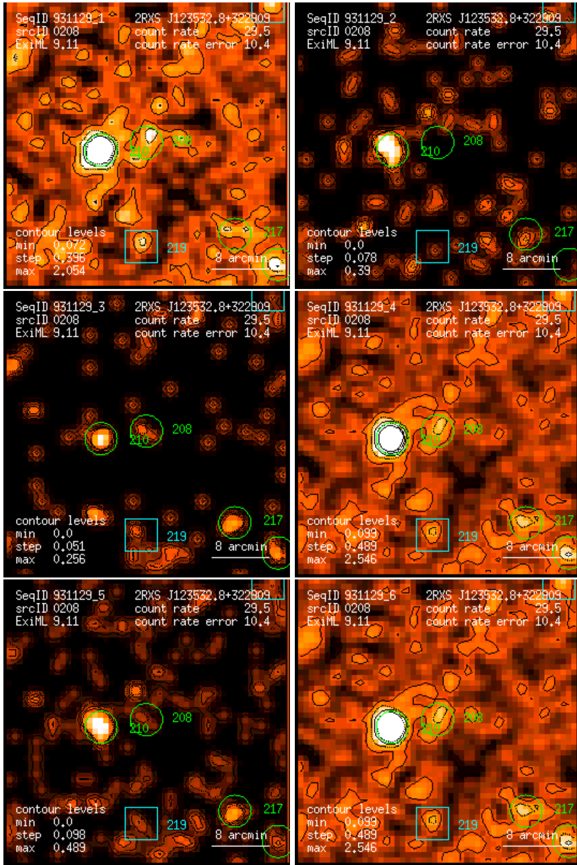
Figure 208: RASS 931129: detection 0208: band rate images, Gaussian filter: (1) PSPC channels 11 – 41, (2) 52 – 90, (3) 91 – 201, (4) 11 – 235, (5) 52 – 201, (6) 11 – 201. Broad band rates in counts/ks. Band rate contour levels in counts/ks/arcmin 2 .
