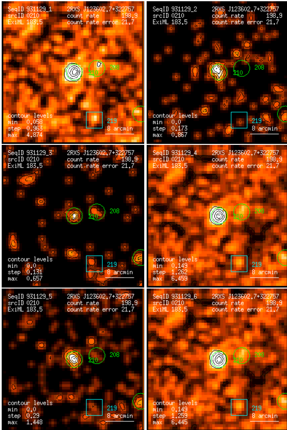
Figure 210: RASS 931129: detection 0210: band rate images, Gaussian filter: (1) PSPC channels 11 – 41, (2) 52 – 90, (3) 91 – 201, (4) 11 – 235, (5) 52 – 201, (6) 11 – 201. Broad band rates in counts/ks. Band rate contour levels in counts/ks/arcmin 2 .
