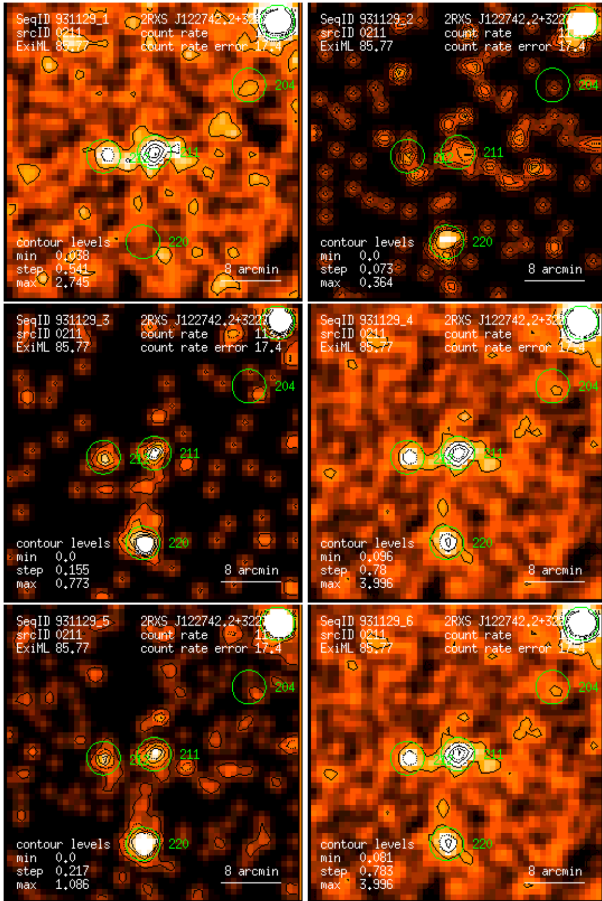
Figure 211: RASS 931129: detection 0211: band rate images, Gaussian filter: (1) PSPC channels 11 – 41, (2) 52 – 90, (3) 91 – 201, (4) 11 – 235, (5) 52 – 201, (6) 11 – 201. Broad band rates in counts/ks. Band rate contour levels in counts/ks/arcmin 2 .
