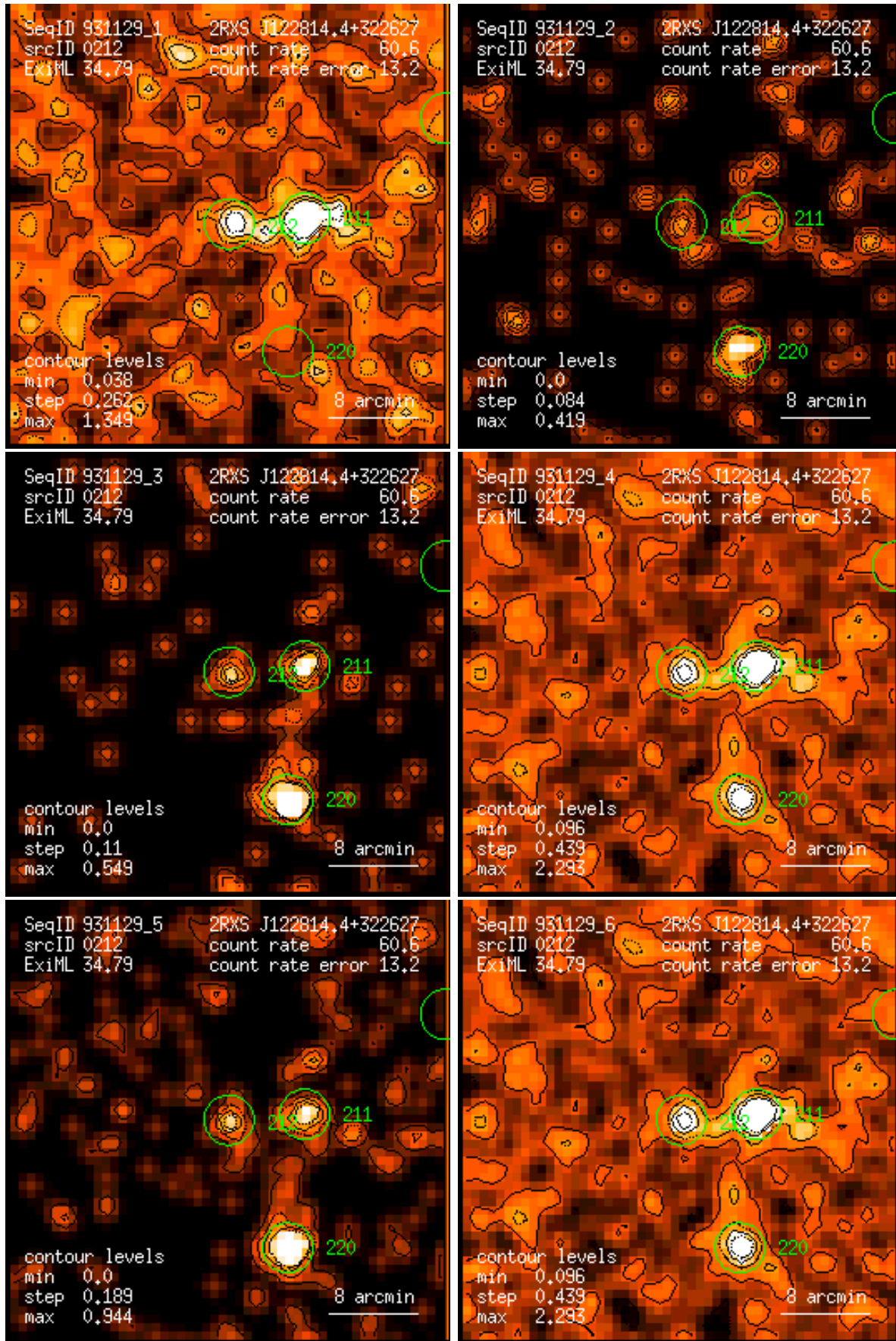
Figure 212: RASS 931129: detection 0212: band rate images, Gaussian filter: (1) PSPC channels 11 – 41, (2) 52 – 90, (3) 91 – 201, (4) 11 – 235, (5) 52 – 201, (6) 11 – 201. Broad band rates in counts/ks. Band rate contour levels in counts/ks/arcmin 2 .
