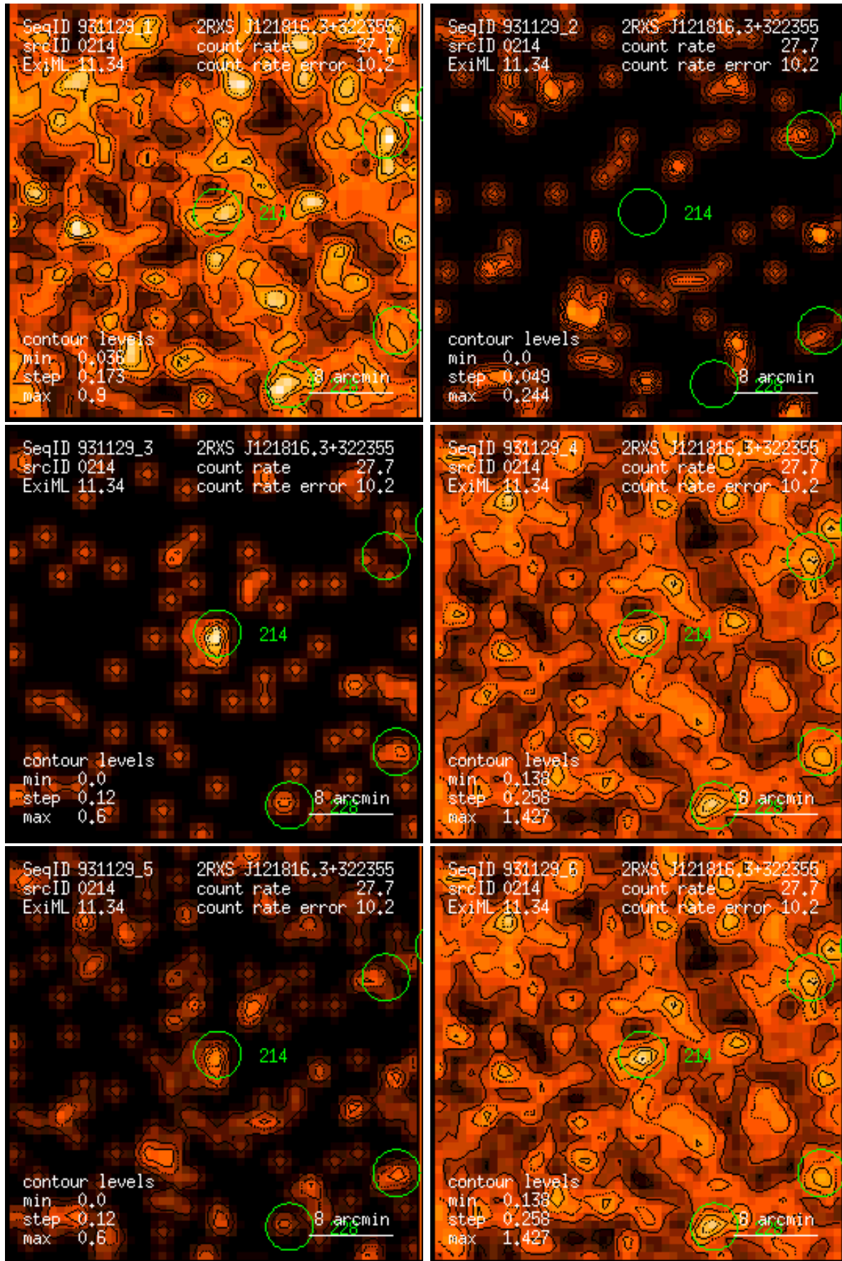
Figure 214: RASS 931129: detection 0214: band rate images, Gaussian filter: (1) PSPC channels 11 – 41, (2) 52 – 90, (3) 91 – 201, (4) 11 – 235, (5) 52 – 201, (6) 11 – 201. Broad band rates in counts/ks. Band rate contour levels in counts/ks/arcmin 2 .
