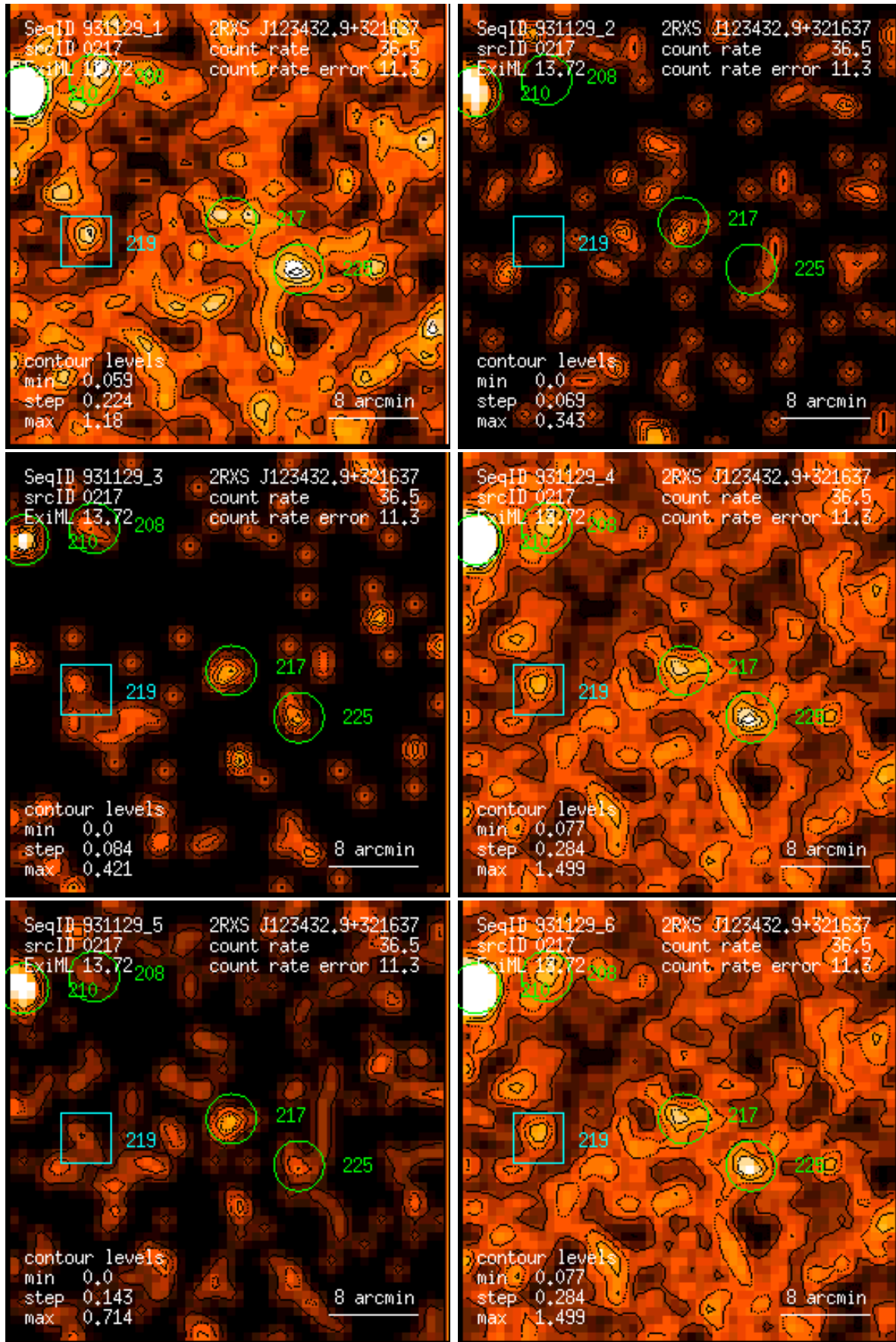
Figure 217: RASS 931129: detection 0217: band rate images, Gaussian filter: (1) PSPC channels 11 – 41, (2) 52 – 90, (3) 91 – 201, (4) 11 – 235, (5) 52 – 201, (6) 11 – 201. Broad band rates in counts/ks. Band rate contour levels in counts/ks/arcmin 2 .
