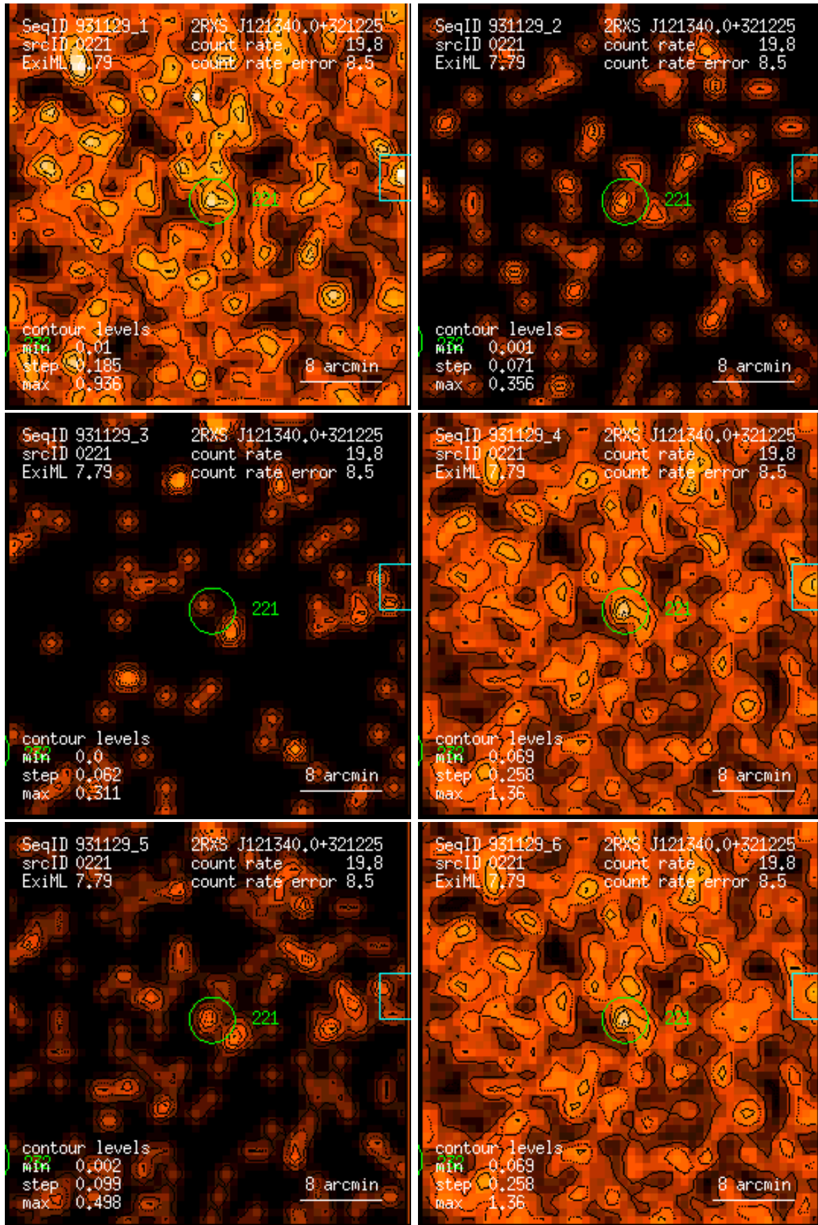
Figure 221: RASS 931129: detection 0221: band rate images, Gaussian filter: (1) PSPC channels 11 – 41, (2) 52 – 90, (3) 91 – 201, (4) 11 – 235, (5) 52 – 201, (6) 11 – 201. Broad band rates in counts/ks. Band rate contour levels in counts/ks/arcmin 2 .
