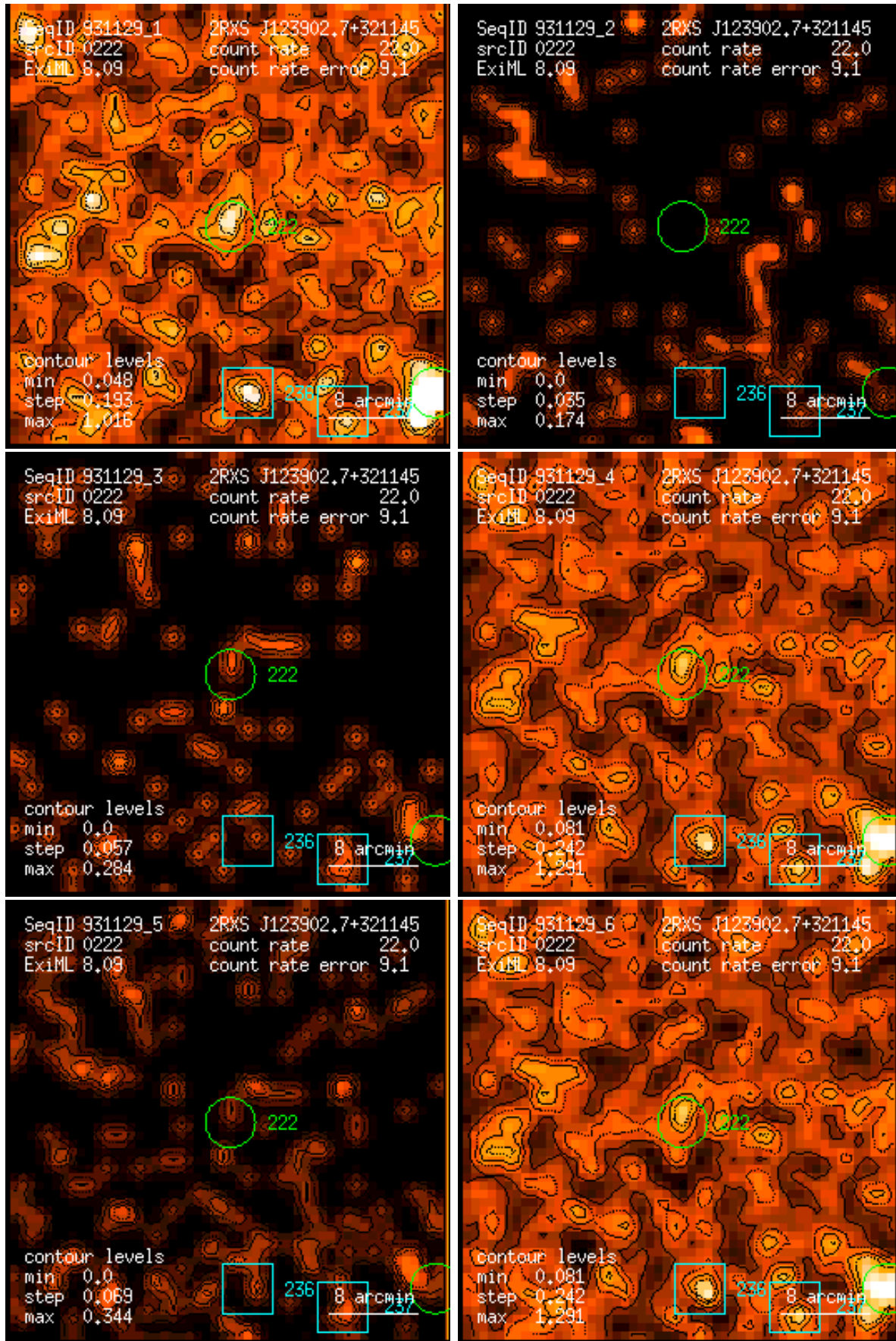
Figure 222: RASS 931129: detection 0222: band rate images, Gaussian filter: (1) PSPC channels 11 – 41, (2) 52 – 90, (3) 91 – 201, (4) 11 – 235, (5) 52 – 201, (6) 11 – 201. Broad band rates in counts/ks. Band rate contour levels in counts/ks/arcmin 2 .
