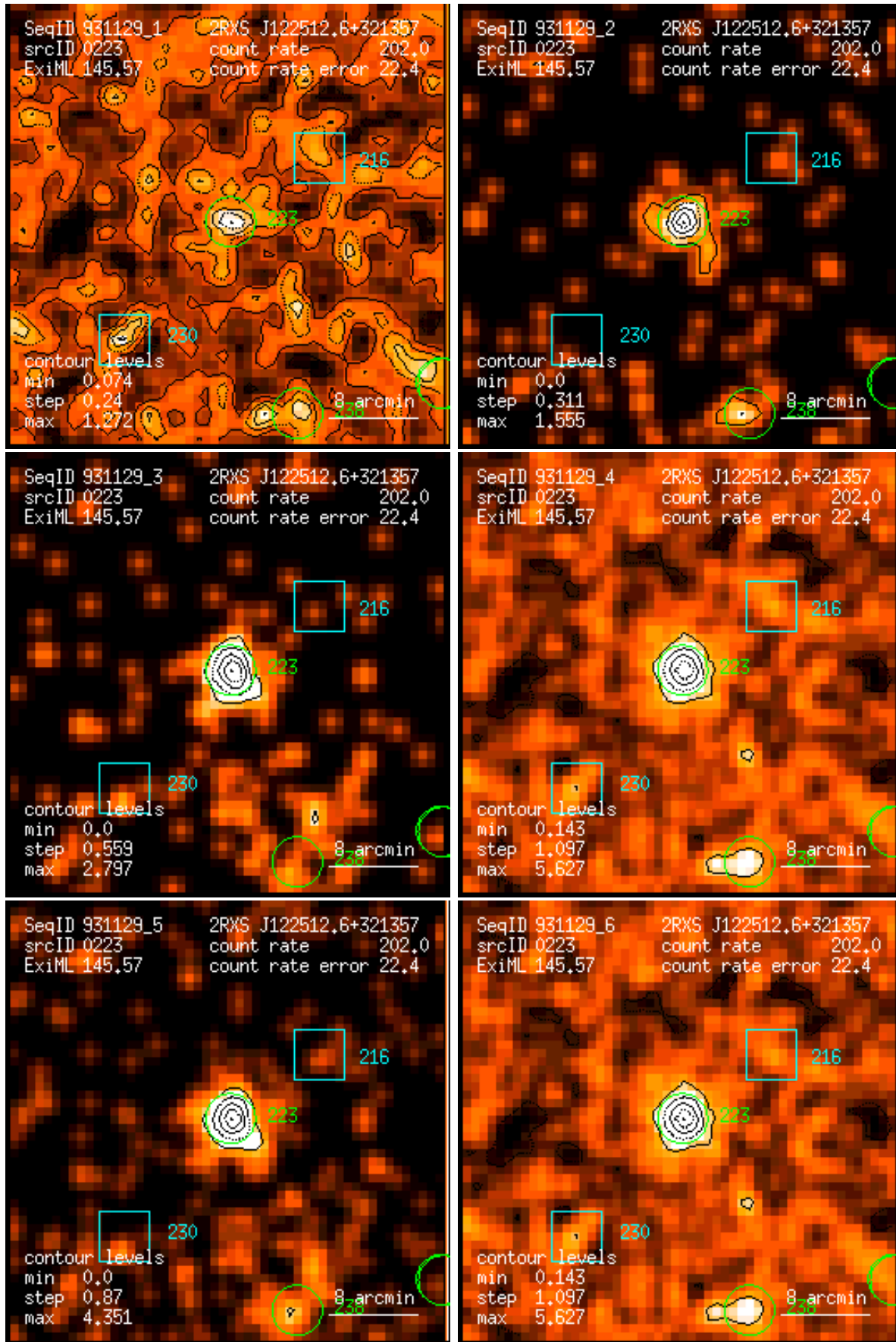
Figure 223: RASS 931129: detection 0223: band rate images, Gaussian filter: (1) PSPC channels 11 – 41, (2) 52 – 90, (3) 91 – 201, (4) 11 – 235, (5) 52 – 201, (6) 11 – 201. Broad band rates in counts/ks. Band rate contour levels in counts/ks/arcmin 2 .
