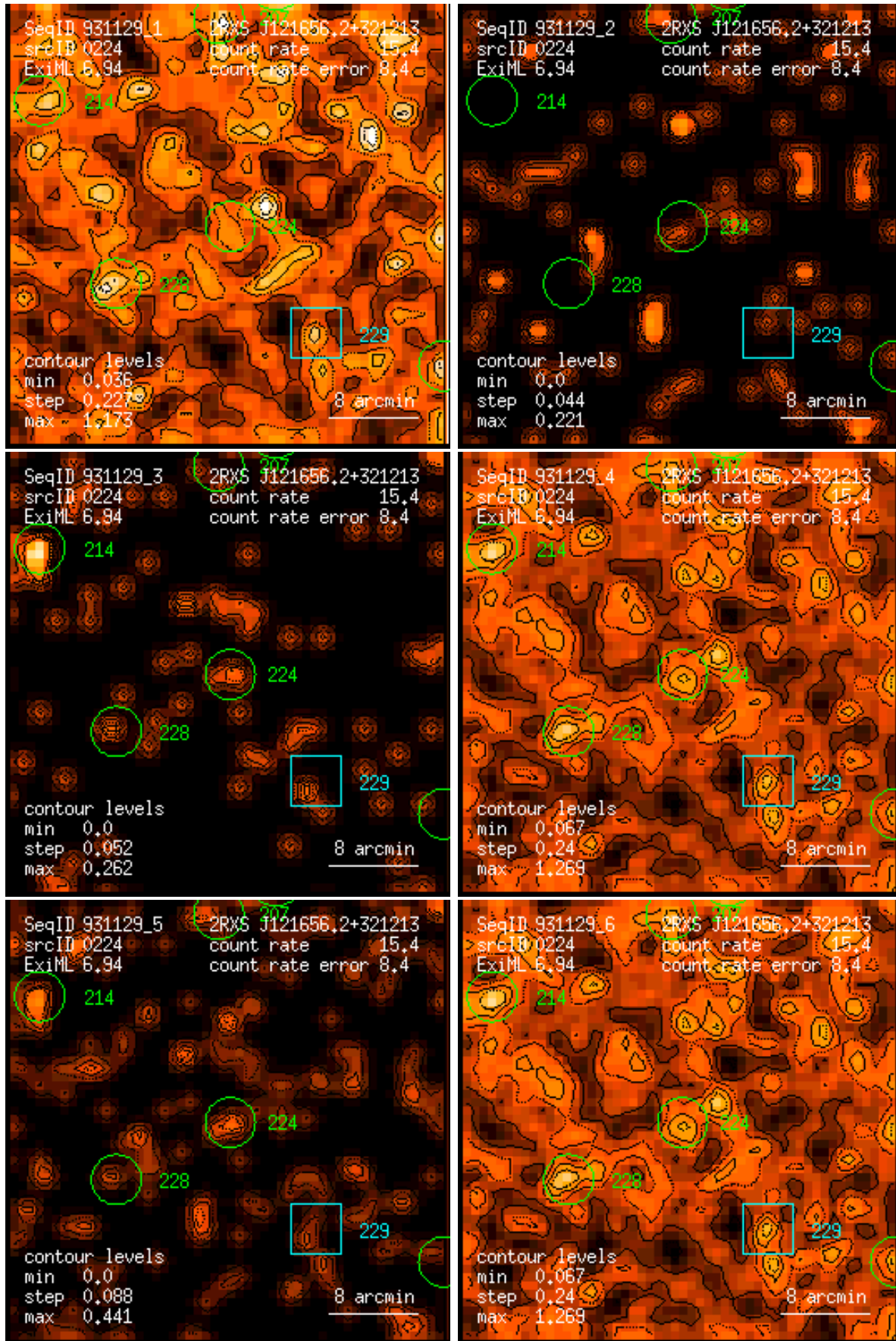
Figure 224: RASS 931129: detection 0224: band rate images, Gaussian filter: (1) PSPC channels 11 – 41, (2) 52 – 90, (3) 91 – 201, (4) 11 – 235, (5) 52 – 201, (6) 11 – 201. Broad band rates in counts/ks. Band rate contour levels in counts/ks/arcmin 2 .
