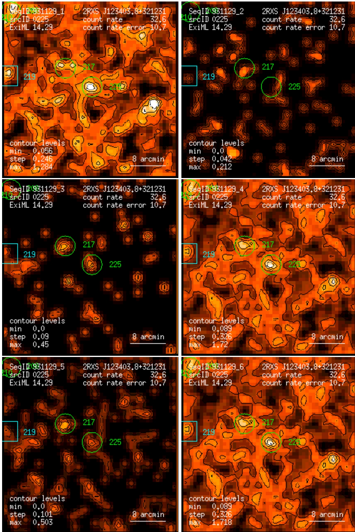
Figure 225: RASS 931129: detection 0225: band rate images, Gaussian filter: (1) PSPC channels 11 – 41, (2) 52 – 90, (3) 91 – 201, (4) 11 – 235, (5) 52 – 201, (6) 11 – 201. Broad band rates in counts/ks. Band rate contour levels in counts/ks/arcmin 2 .
