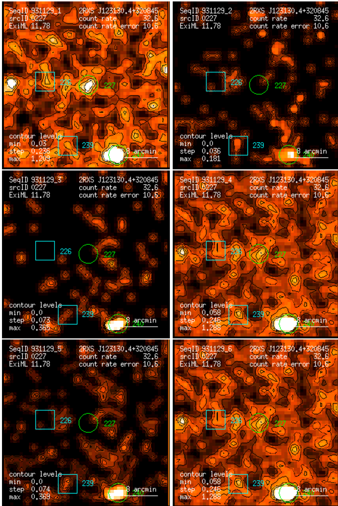
Figure 227: RASS 931129: detection 0227: band rate images, Gaussian filter: (1) PSPC channels 11 – 41, (2) 52 – 90, (3) 91 – 201, (4) 11 – 235, (5) 52 – 201, (6) 11 – 201. Broad band rates in counts/ks. Band rate contour levels in counts/ks/arcmin 2 .
