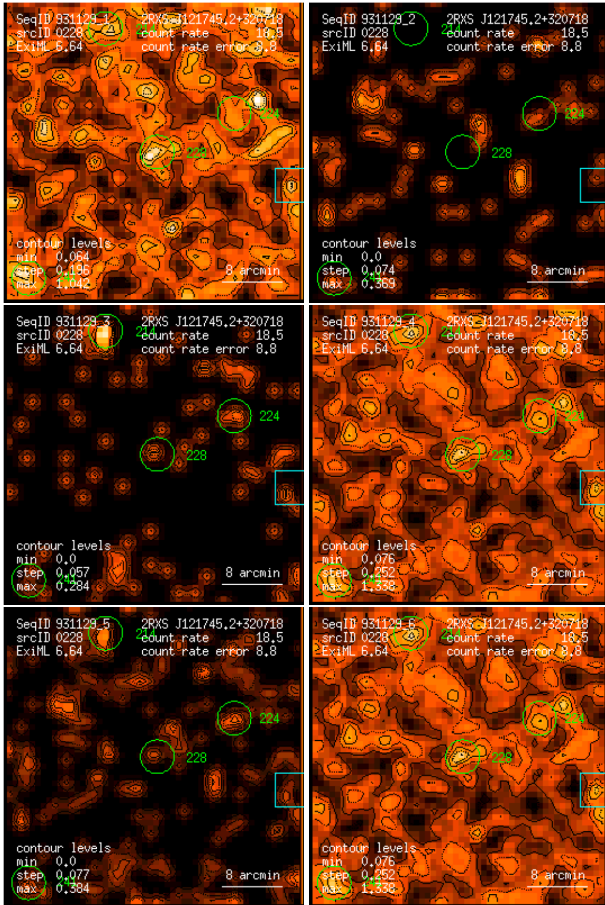
Figure 228: RASS 931129: detection 0228: band rate images, Gaussian filter: (1) PSPC channels 11 – 41, (2) 52 – 90, (3) 91 – 201, (4) 11 – 235, (5) 52 – 201, (6) 11 – 201. Broad band rates in counts/ks. Band rate contour levels in counts/ks/arcmin 2 .
