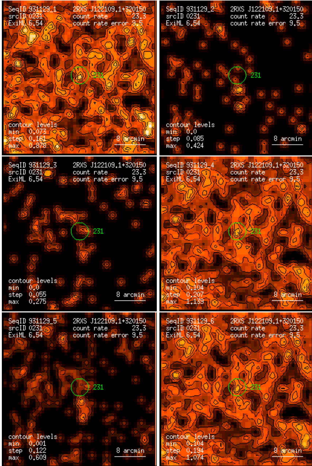
Figure 231: RASS 931129: detection 0231: band rate images, Gaussian filter: (1) PSPC channels 11 – 41, (2) 52 – 90, (3) 91 – 201, (4) 11 – 235, (5) 52 – 201, (6) 11 – 201. Broad band rates in counts/ks. Band rate contour levels in counts/ks/arcmin 2 .
