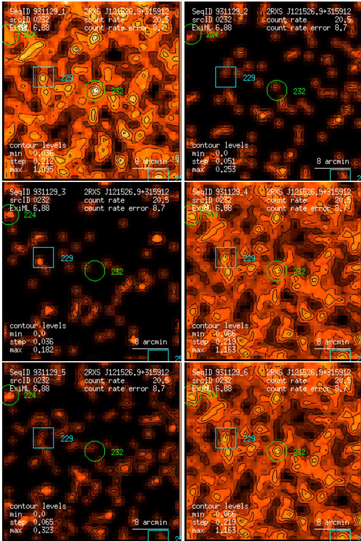
Figure 232: RASS 931129: detection 0232: band rate images, Gaussian filter: (1) PSPC channels 11 – 41, (2) 52 – 90, (3) 91 – 201, (4) 11 – 235, (5) 52 – 201, (6) 11 – 201. Broad band rates in counts/ks. Band rate contour levels in counts/ks/arcmin 2 .
