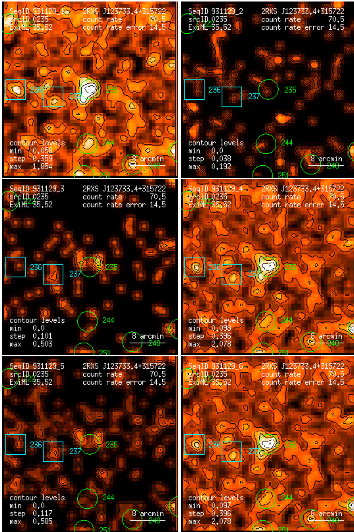
Figure 235: RASS 931129: detection 0235: band rate images, Gaussian filter: (1) PSPC channels 11 – 41, (2) 52 – 90, (3) 91 – 201, (4) 11 – 235, (5) 52 – 201, (6) 11 – 201. Broad band rates in counts/ks. Band rate contour levels in counts/ks/arcmin 2 .
