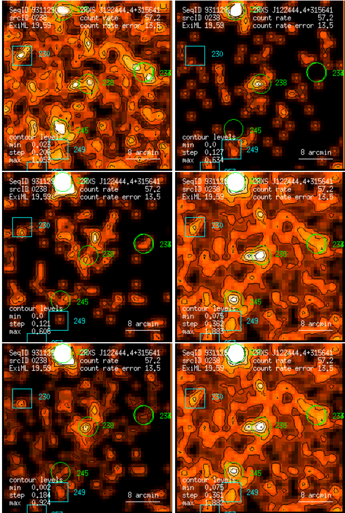
Figure 238: RASS 931129: detection 0238: band rate images, Gaussian filter: (1) PSPC channels 11 – 41, (2) 52 – 90, (3) 91 – 201, (4) 11 – 235, (5) 52 – 201, (6) 11 – 201. Broad band rates in counts/ks. Band rate contour levels in counts/ks/arcmin 2 .
