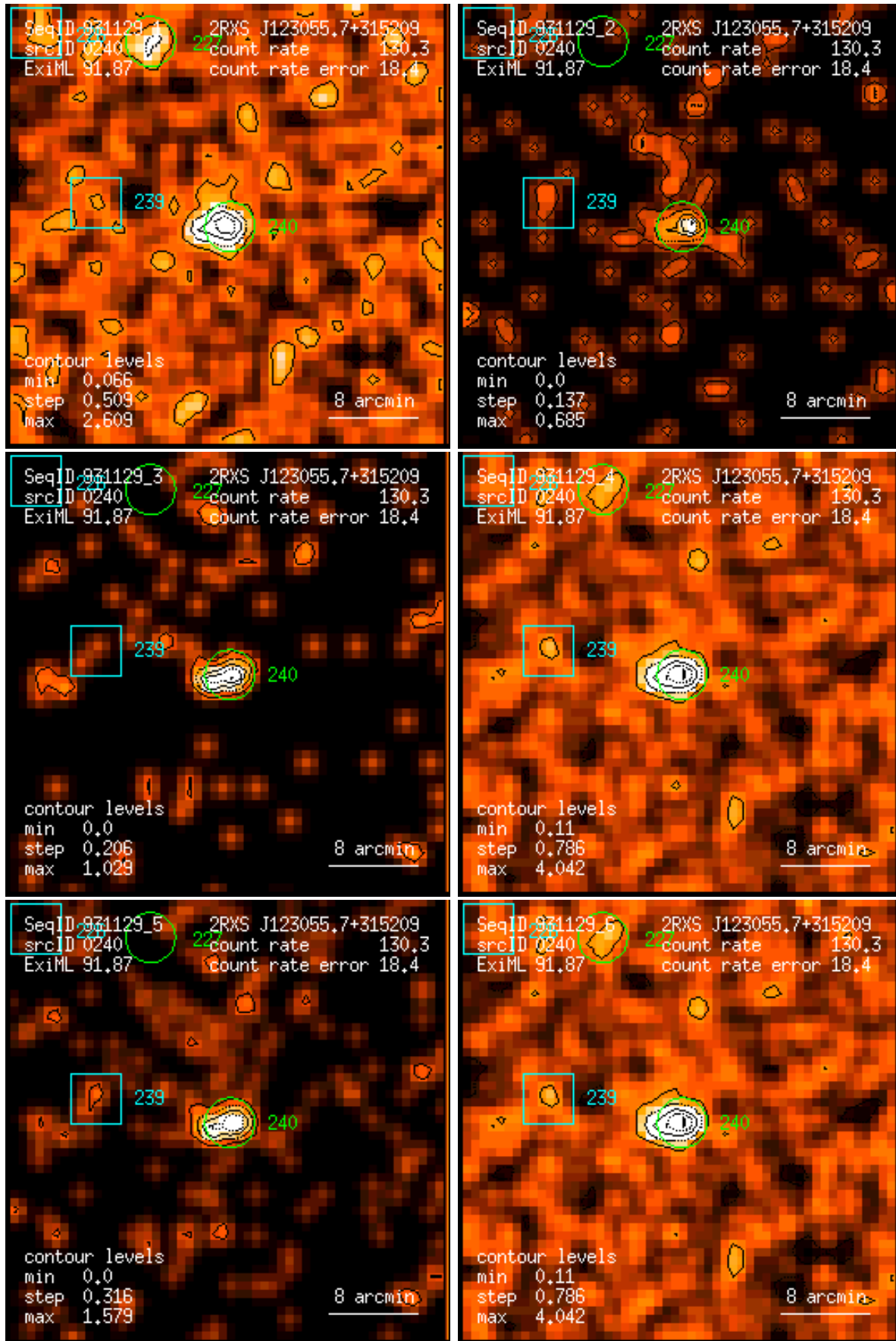
Figure 240: RASS 931129: detection 0240: band rate images, Gaussian filter: (1) PSPC channels 11 – 41, (2) 52 – 90, (3) 91 – 201, (4) 11 – 235, (5) 52 – 201, (6) 11 – 201. Broad band rates in counts/ks. Band rate contour levels in counts/ks/arcmin 2 .
