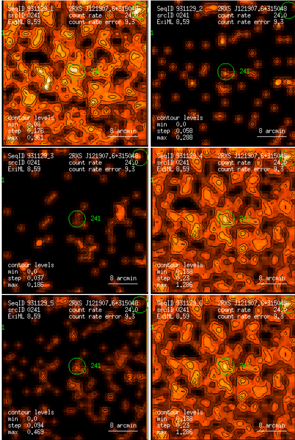
Figure 241: RASS 931129: detection 0241: band rate images, Gaussian filter: (1) PSPC channels 11 – 41, (2) 52 – 90, (3) 91 – 201, (4) 11 – 235, (5) 52 – 201, (6) 11 – 201. Broad band rates in counts/ks. Band rate contour levels in counts/ks/arcmin 2 .
