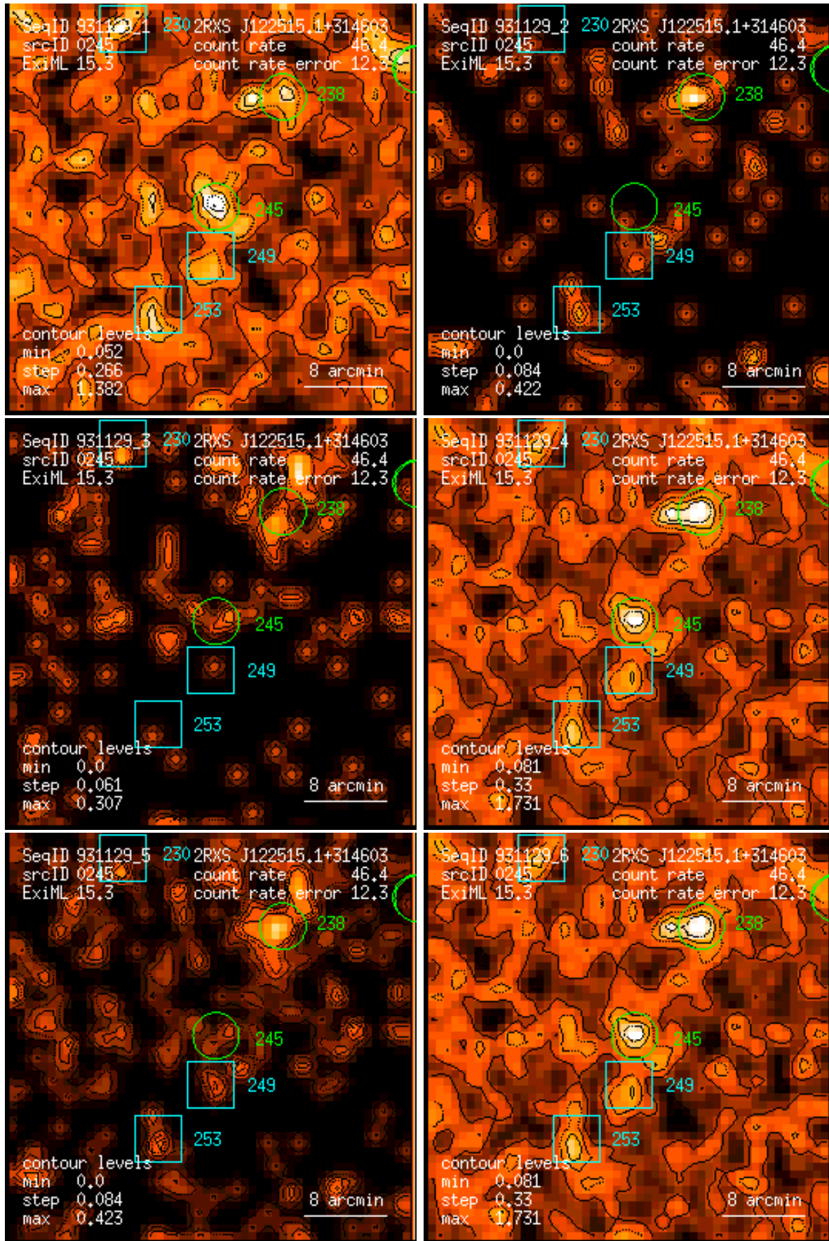
Figure 245: RASS 931129: detection 0245: band rate images, Gaussian filter: (1) PSPC channels 11 – 41, (2) 52 – 90, (3) 91 – 201, (4) 11 – 235, (5) 52 – 201, (6) 11 – 201. Broad band rates in counts/ks. Band rate contour levels in counts/ks/arcmin 2 .
