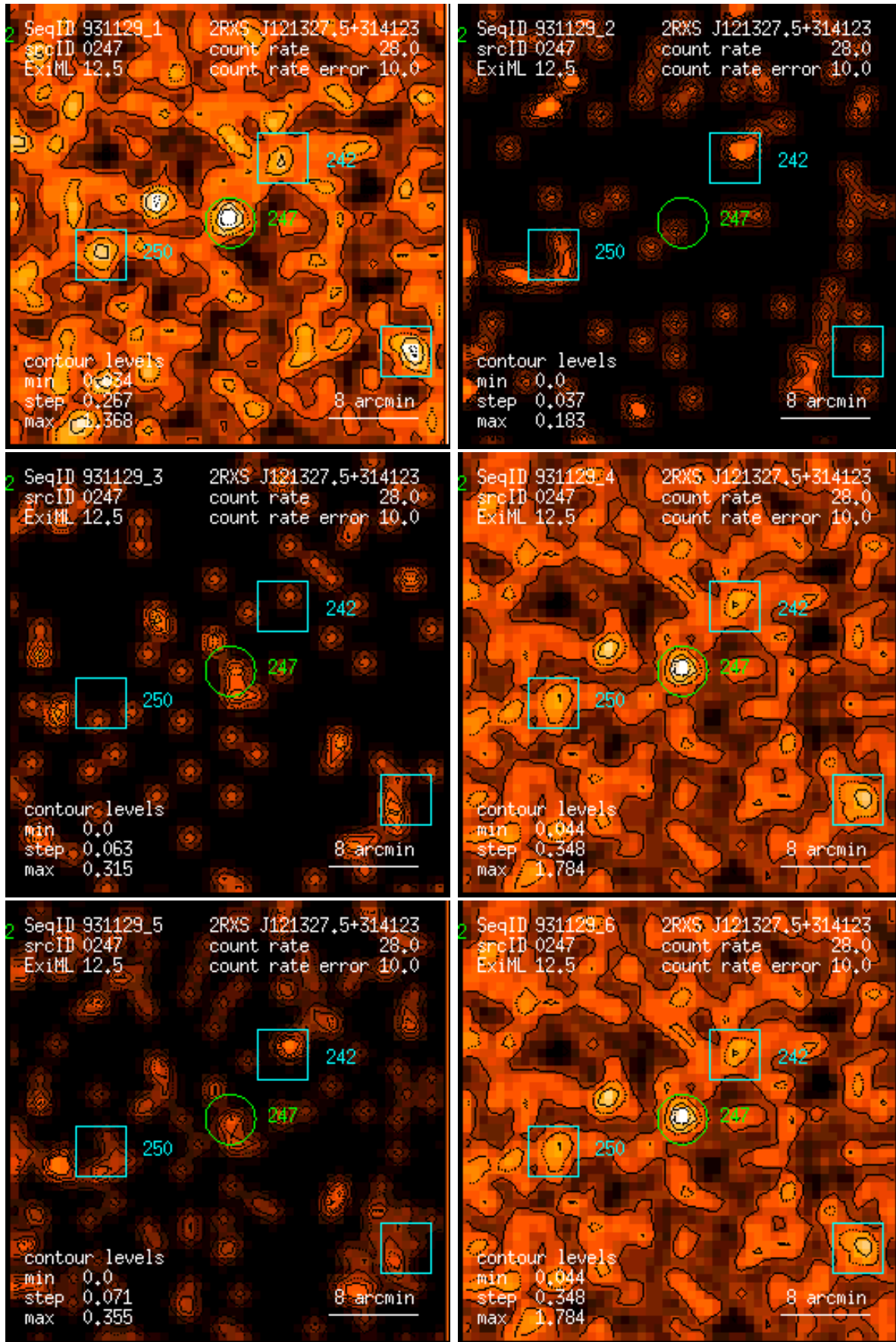
Figure 247: RASS 931129: detection 0247: band rate images, Gaussian filter: (1) PSPC channels 11 – 41, (2) 52 – 90, (3) 91 – 201, (4) 11 – 235, (5) 52 – 201, (6) 11 – 201. Broad band rates in counts/ks. Band rate contour levels in counts/ks/arcmin 2 .
