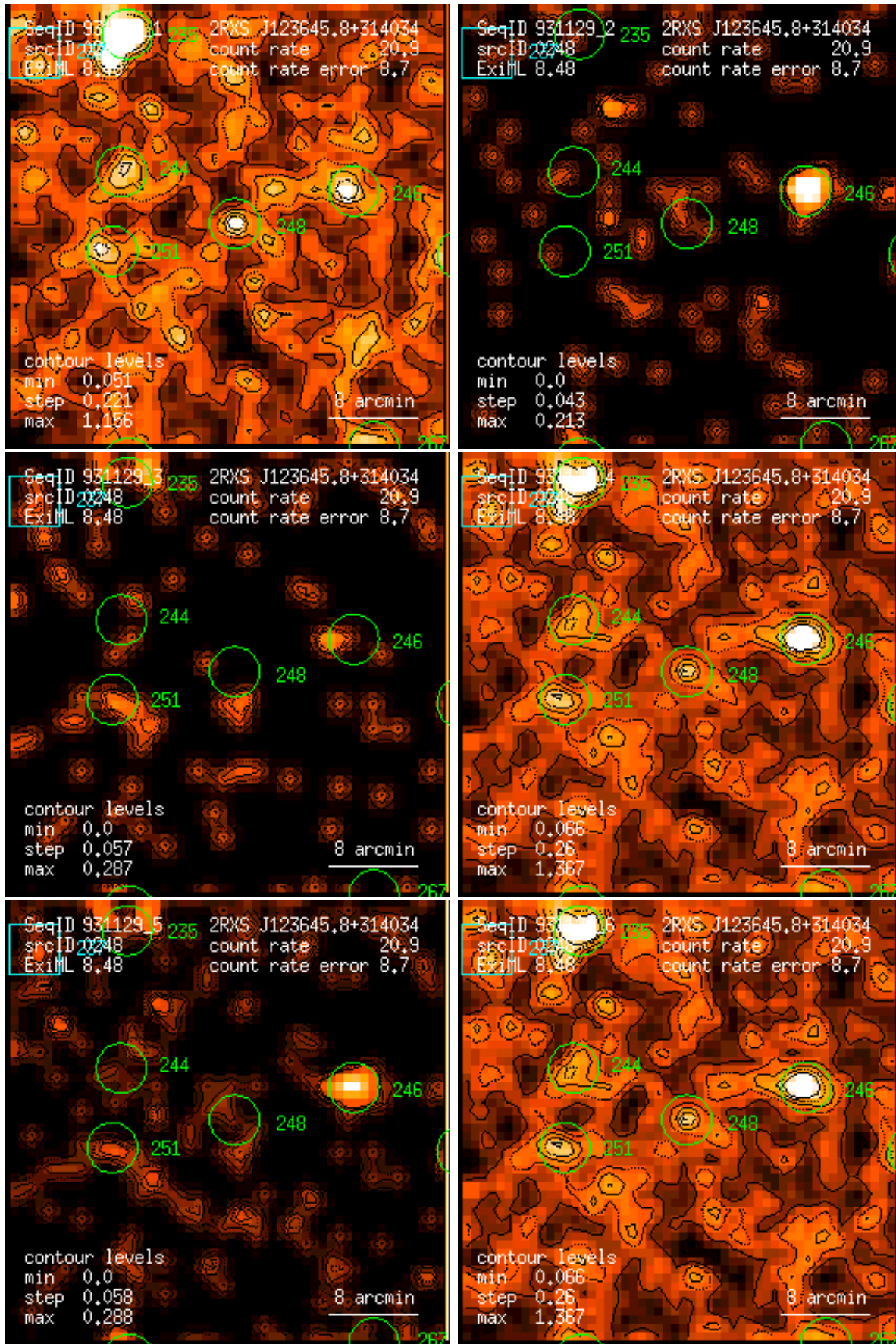
Figure 248: RASS 931129: detection 0248: band rate images, Gaussian filter: (1) PSPC channels 11 – 41, (2) 52 – 90, (3) 91 – 201, (4) 11 – 235, (5) 52 – 201, (6) 11 – 201. Broad band rates in counts/ks. Band rate contour levels in counts/ks/arcmin 2 .
