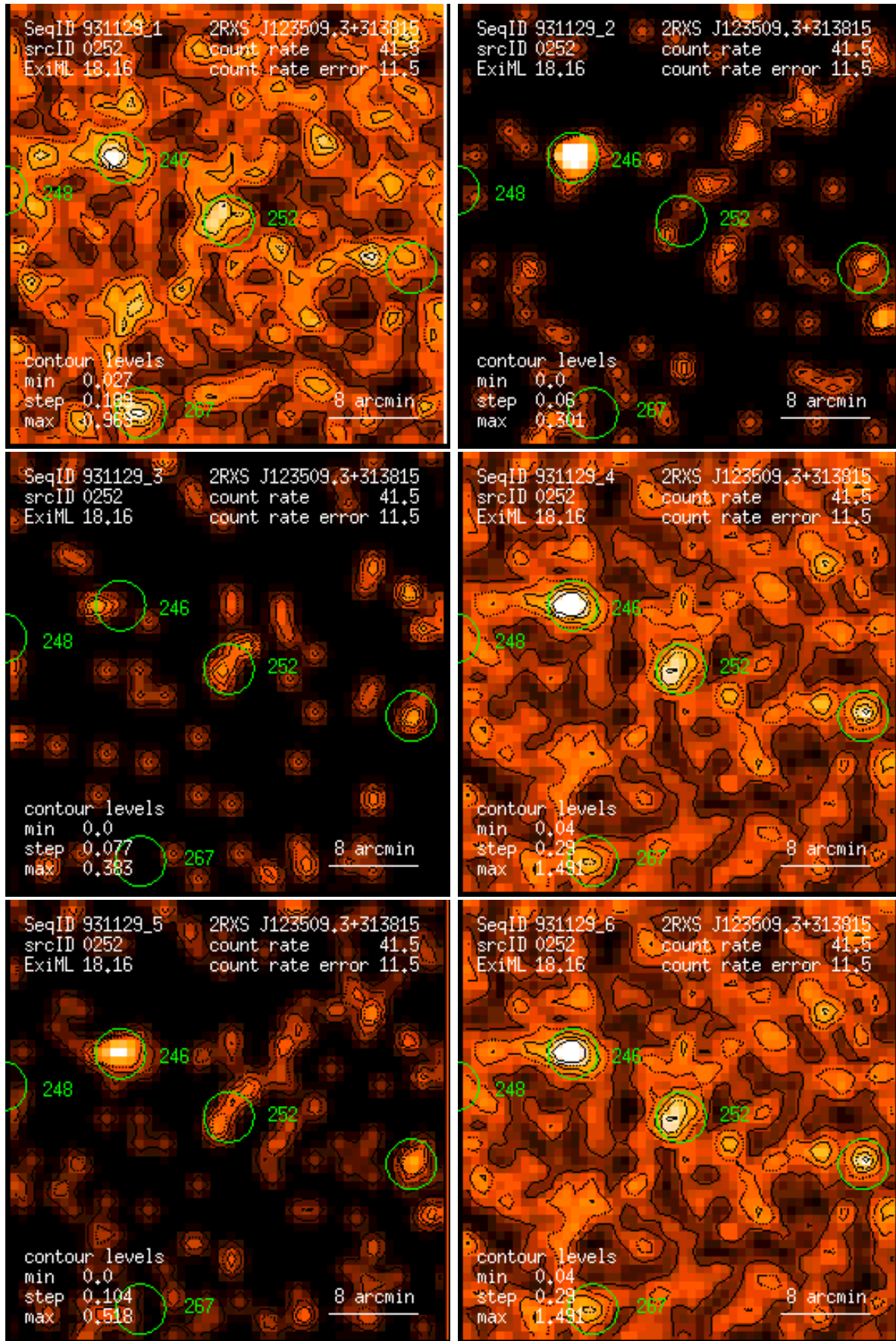
Figure 252: RASS 931129: detection 0252: band rate images, Gaussian filter: (1) PSPC channels 11 – 41, (2) 52 – 90, (3) 91 – 201, (4) 11 – 235, (5) 52 – 201, (6) 11 – 201. Broad band rates in counts/ks. Band rate contour levels in counts/ks/arcmin 2 .
