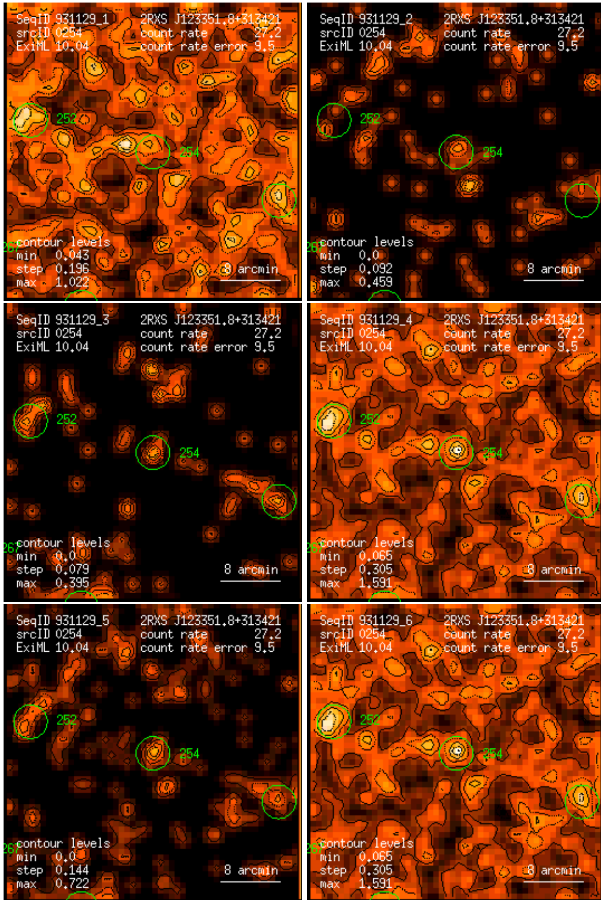
Figure 254: RASS 931129: detection 0254: band rate images, Gaussian filter: (1) PSPC channels 11 – 41, (2) 52 – 90, (3) 91 – 201, (4) 11 – 235, (5) 52 – 201, (6) 11 – 201. Broad band rates in counts/ks. Band rate contour levels in counts/ks/arcmin 2 .
