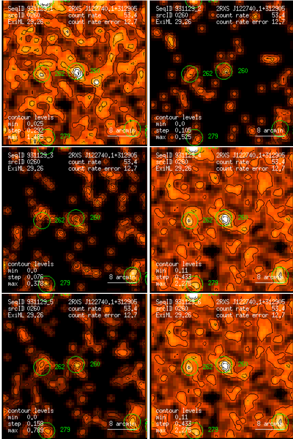
Figure 260: RASS 931129: detection 0260: band rate images, Gaussian filter: (1) PSPC channels 11 – 41, (2) 52 – 90, (3) 91 – 201, (4) 11 – 235, (5) 52 – 201, (6) 11 – 201. Broad band rates in counts/ks. Band rate contour levels in counts/ks/arcmin 2 .
