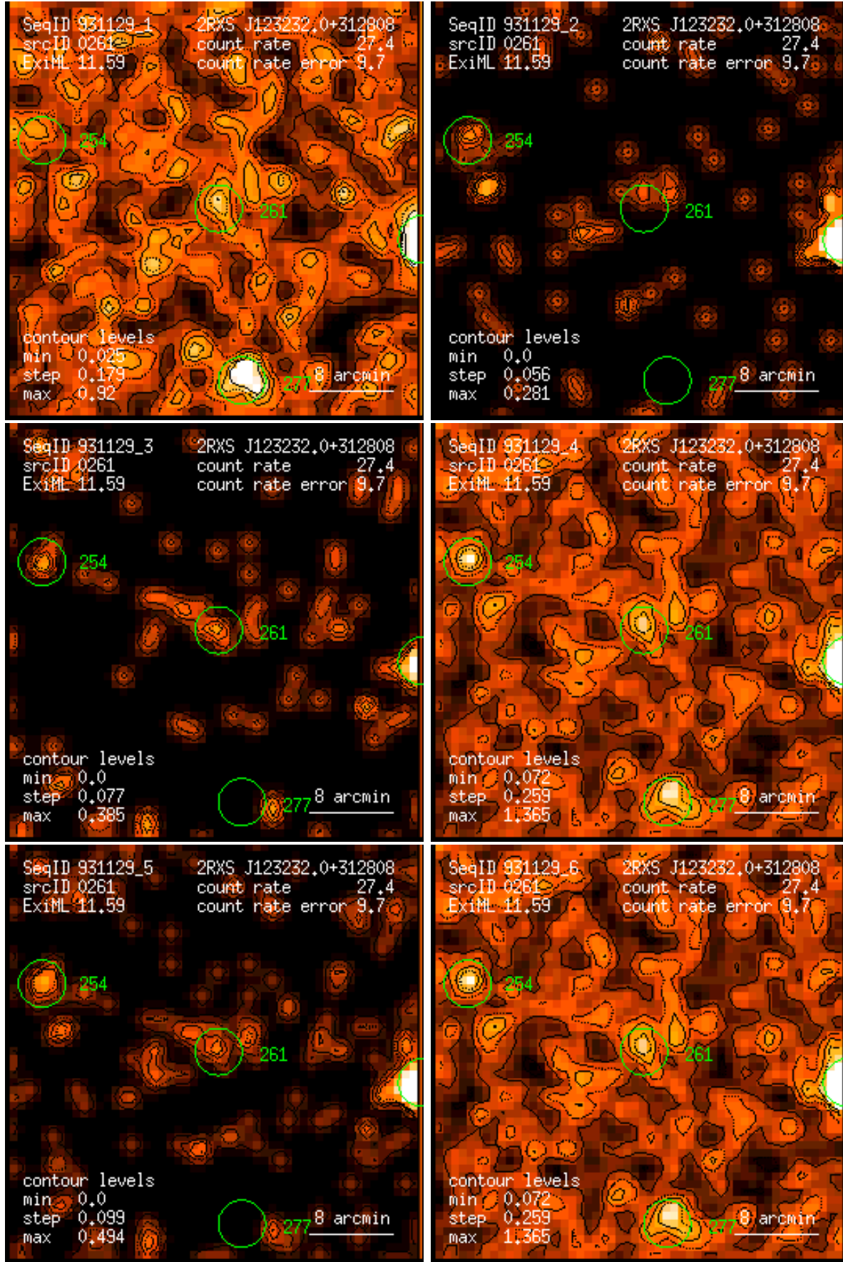
Figure 261: RASS 931129: detection 0261: band rate images, Gaussian filter: (1) PSPC channels 11 – 41, (2) 52 – 90, (3) 91 – 201, (4) 11 – 235, (5) 52 – 201, (6) 11 – 201. Broad band rates in counts/ks. Band rate contour levels in counts/ks/arcmin 2 .
