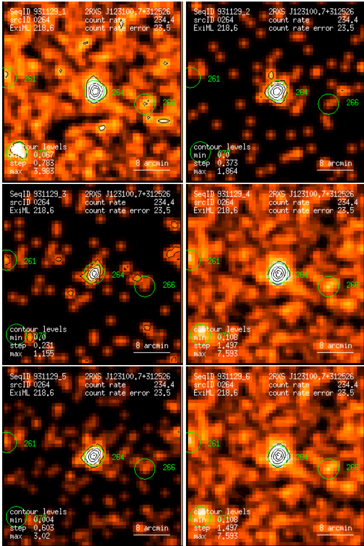
Figure 264: RASS 931129: detection 0264: band rate images, Gaussian filter: (1) PSPC channels 11 – 41, (2) 52 – 90, (3) 91 – 201, (4) 11 – 235, (5) 52 – 201, (6) 11 – 201. Broad band rates in counts/ks. Band rate contour levels in counts/ks/arcmin 2 .
