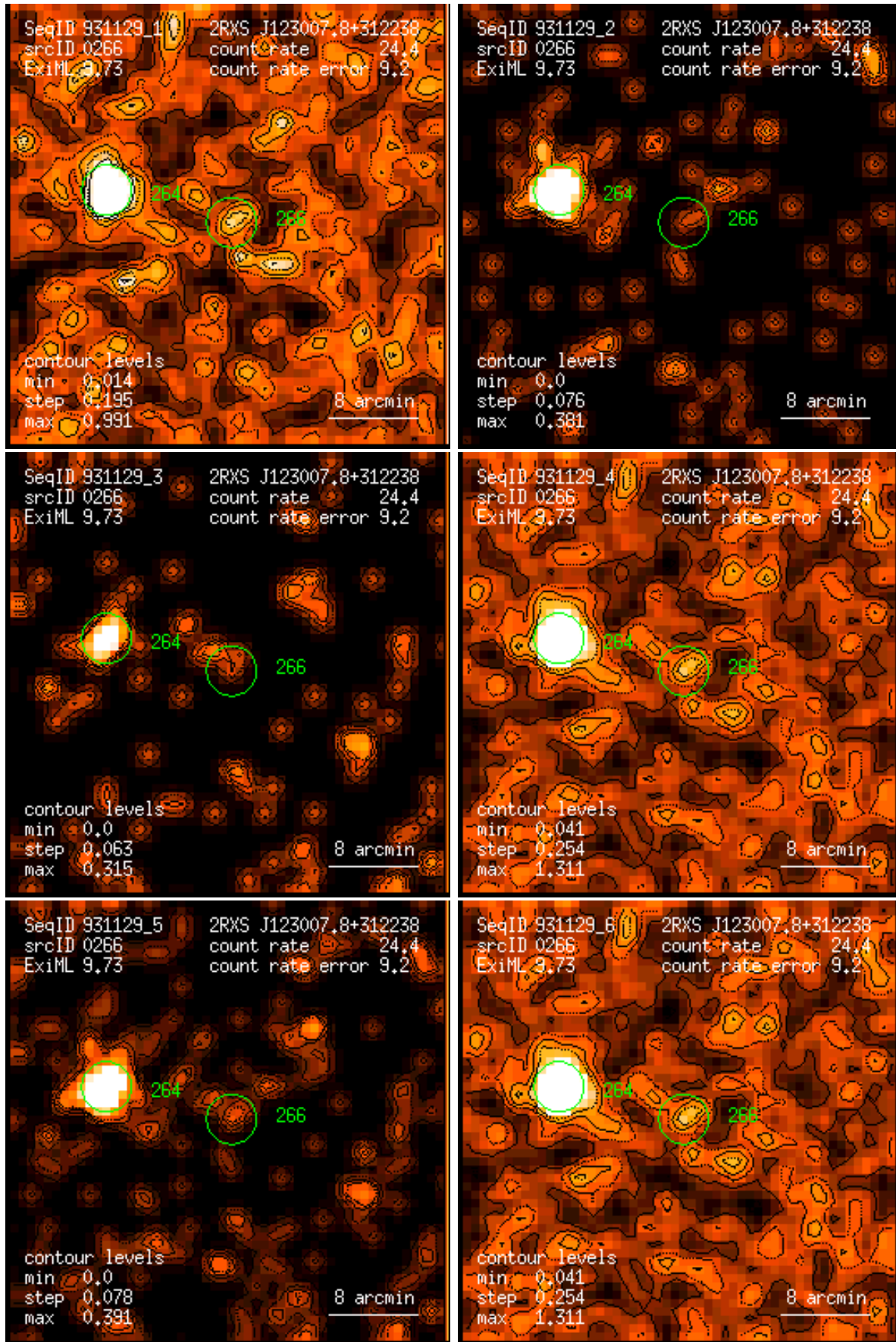
Figure 266: RASS 931129: detection 0266: band rate images, Gaussian filter: (1) PSPC channels 11 – 41, (2) 52 – 90, (3) 91 – 201, (4) 11 – 235, (5) 52 – 201, (6) 11 – 201. Broad band rates in counts/ks. Band rate contour levels in counts/ks/arcmin 2 .
