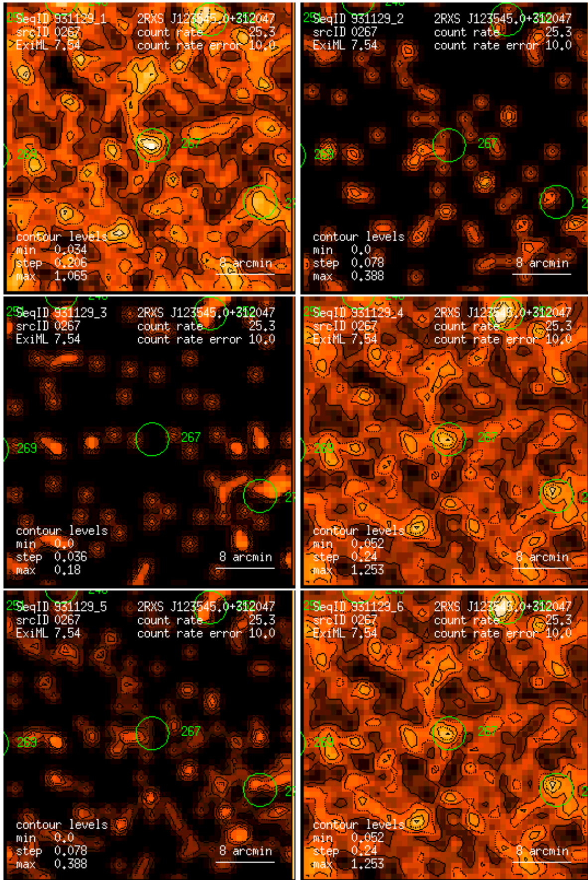
Figure 267: RASS 931129: detection 0267: band rate images, Gaussian filter: (1) PSPC channels 11 – 41, (2) 52 – 90, (3) 91 – 201, (4) 11 – 235, (5) 52 – 201, (6) 11 – 201. Broad band rates in counts/ks. Band rate contour levels in counts/ks/arcmin 2 .
