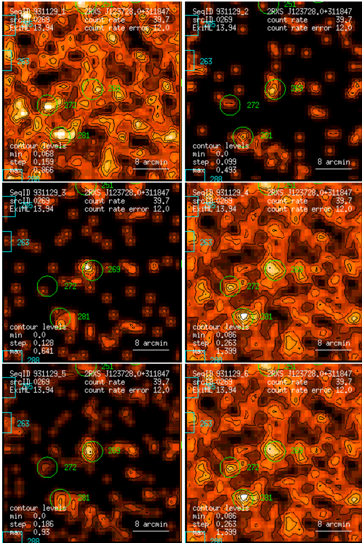
Figure 269: RASS 931129: detection 0269: band rate images, Gaussian filter: (1) PSPC channels 11 – 41, (2) 52 – 90, (3) 91 – 201, (4) 11 – 235, (5) 52 – 201, (6) 11 – 201. Broad band rates in counts/ks. Band rate contour levels in counts/ks/arcmin 2 .
