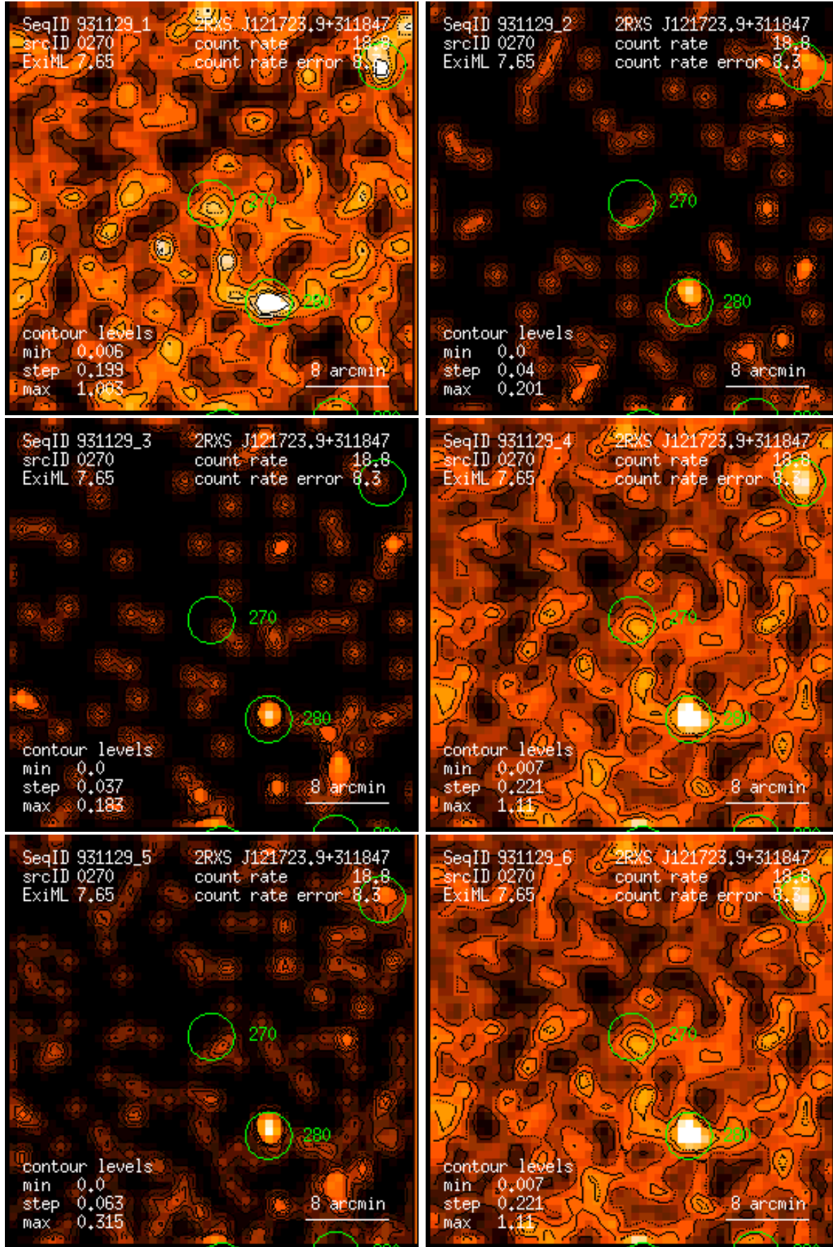
Figure 270: RASS 931129: detection 0270: band rate images, Gaussian filter: (1) PSPC channels 11 – 41, (2) 52 – 90, (3) 91 – 201, (4) 11 – 235, (5) 52 – 201, (6) 11 – 201. Broad band rates in counts/ks. Band rate contour levels in counts/ks/arcmin 2 .
