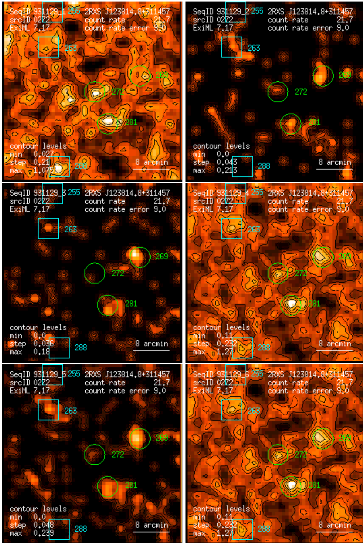
Figure 272: RASS 931129: detection 0272: band rate images, Gaussian filter: (1) PSPC channels 11 – 41, (2) 52 – 90, (3) 91 – 201, (4) 11 – 235, (5) 52 – 201, (6) 11 – 201. Broad band rates in counts/ks. Band rate contour levels in counts/ks/arcmin 2 .
