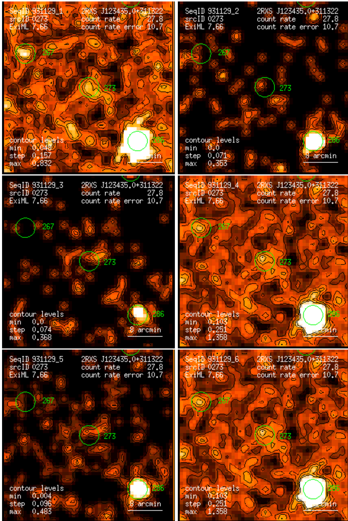
Figure 273: RASS 931129: detection 0273: band rate images, Gaussian filter: (1) PSPC channels 11 – 41, (2) 52 – 90, (3) 91 – 201, (4) 11 – 235, (5) 52 – 201, (6) 11 – 201. Broad band rates in counts/ks. Band rate contour levels in counts/ks/arcmin 2 .
