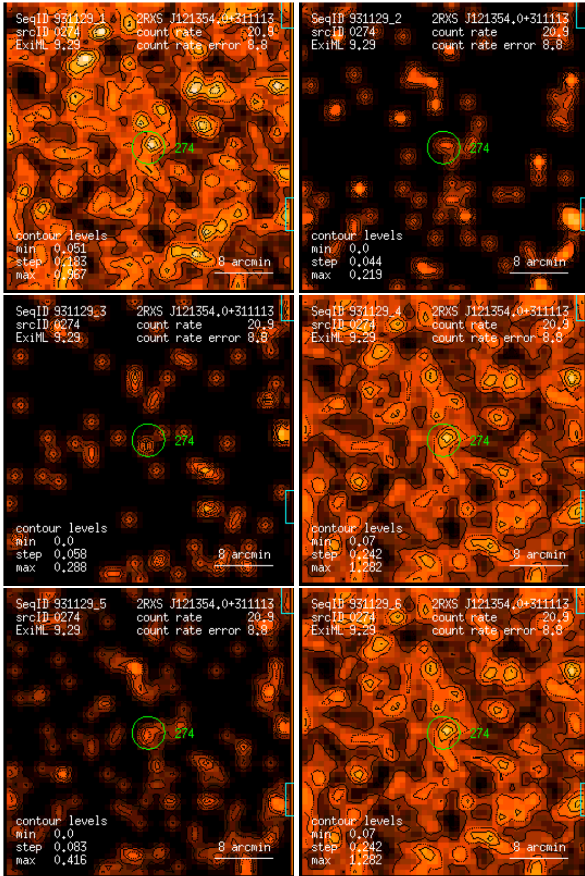
Figure 274: RASS 931129: detection 0274: band rate images, Gaussian filter: (1) PSPC channels 11 – 41, (2) 52 – 90, (3) 91 – 201, (4) 11 – 235, (5) 52 – 201, (6) 11 – 201. Broad band rates in counts/ks. Band rate contour levels in counts/ks/arcmin 2 .
