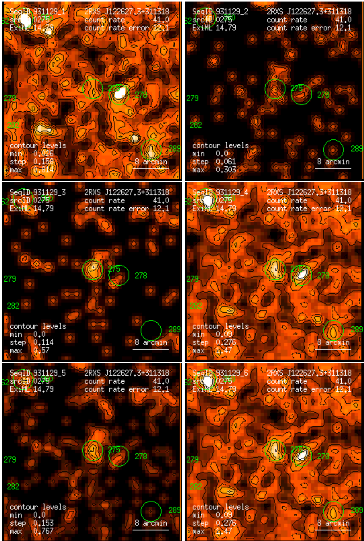
Figure 275: RASS 931129: detection 0275: band rate images, Gaussian filter: (1) PSPC channels 11 – 41, (2) 52 – 90, (3) 91 – 201, (4) 11 – 235, (5) 52 – 201, (6) 11 – 201. Broad band rates in counts/ks. Band rate contour levels in counts/ks/arcmin 2 .
