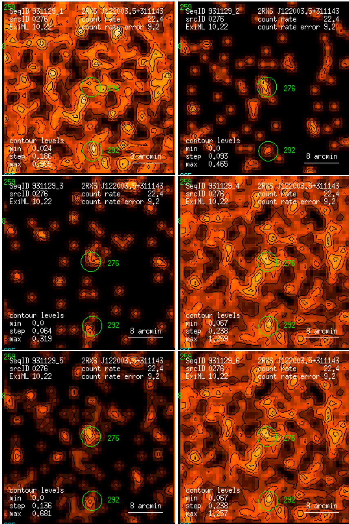
Figure 276: RASS 931129: detection 0276: band rate images, Gaussian filter: (1) PSPC channels 11 – 41, (2) 52 – 90, (3) 91 – 201, (4) 11 – 235, (5) 52 – 201, (6) 11 – 201. Broad band rates in counts/ks. Band rate contour levels in counts/ks/arcmin 2 .
