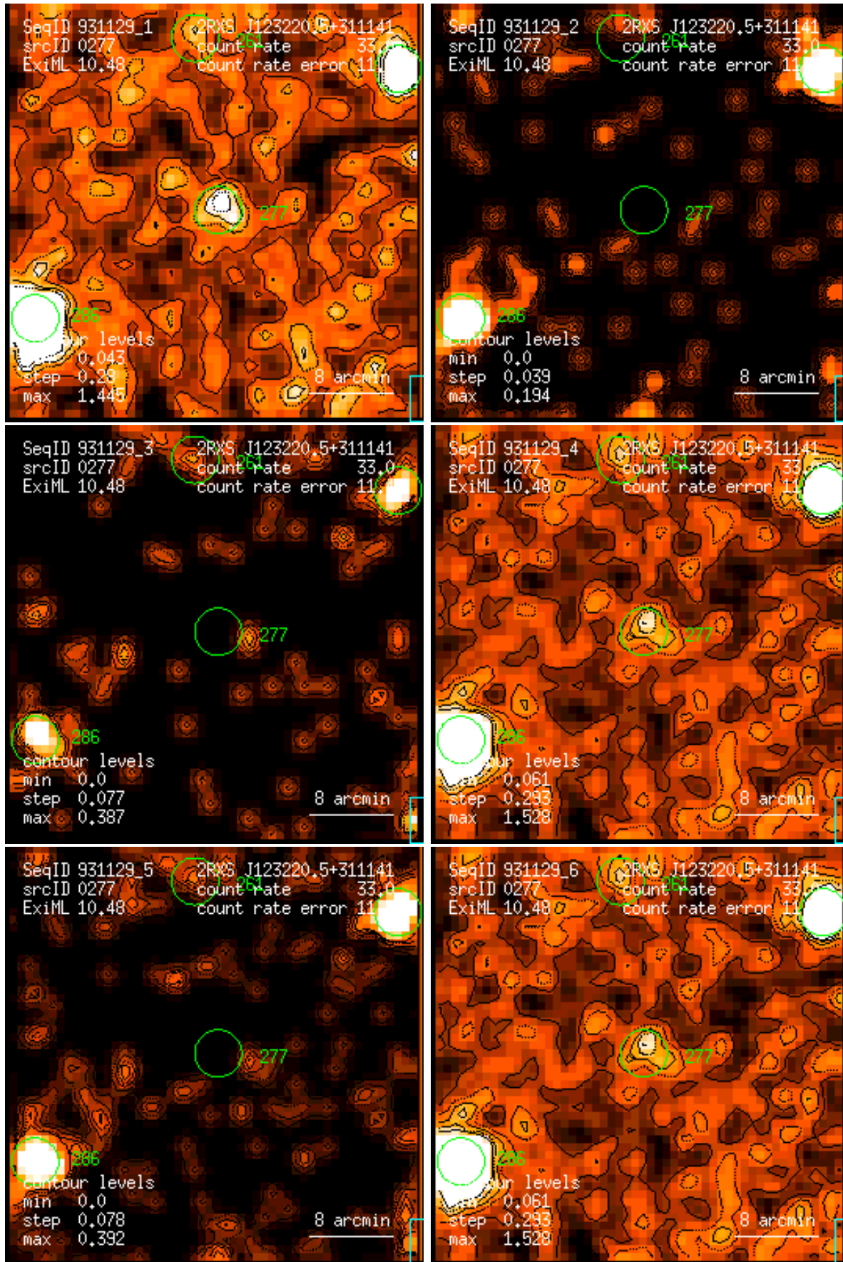
Figure 277: RASS 931129: detection 0277: band rate images, Gaussian filter: (1) PSPPC channels 11 – 41, (2) 52 – 90, (3) 91 – 201, (4) 11 – 235, (5) 52 – 201, (6) 11 – 201. Broad band rates in counts/ks. Band rate contour levels in counts/ks/arcmin 2 .
