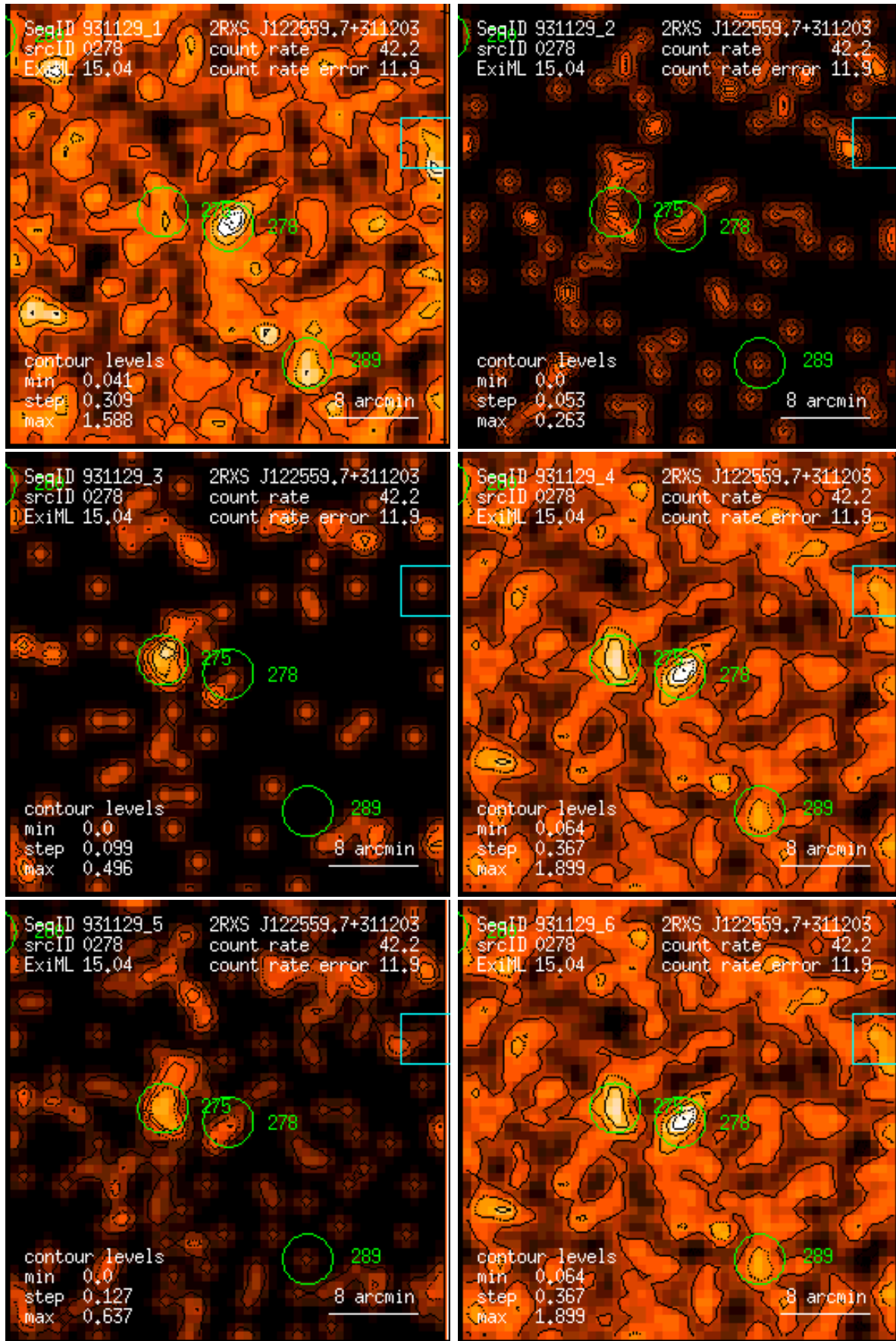
Figure 278: RASS 931129: detection 0278: band rate images, Gaussian filter: (1) PSPC channels 11 – 41, (2) 52 – 90, (3) 91 – 201, (4) 11 – 235, (5) 52 – 201, (6) 11 – 201. Broad band rates in counts/ks. Band rate contour levels in counts/ks/arcmin 2 .
