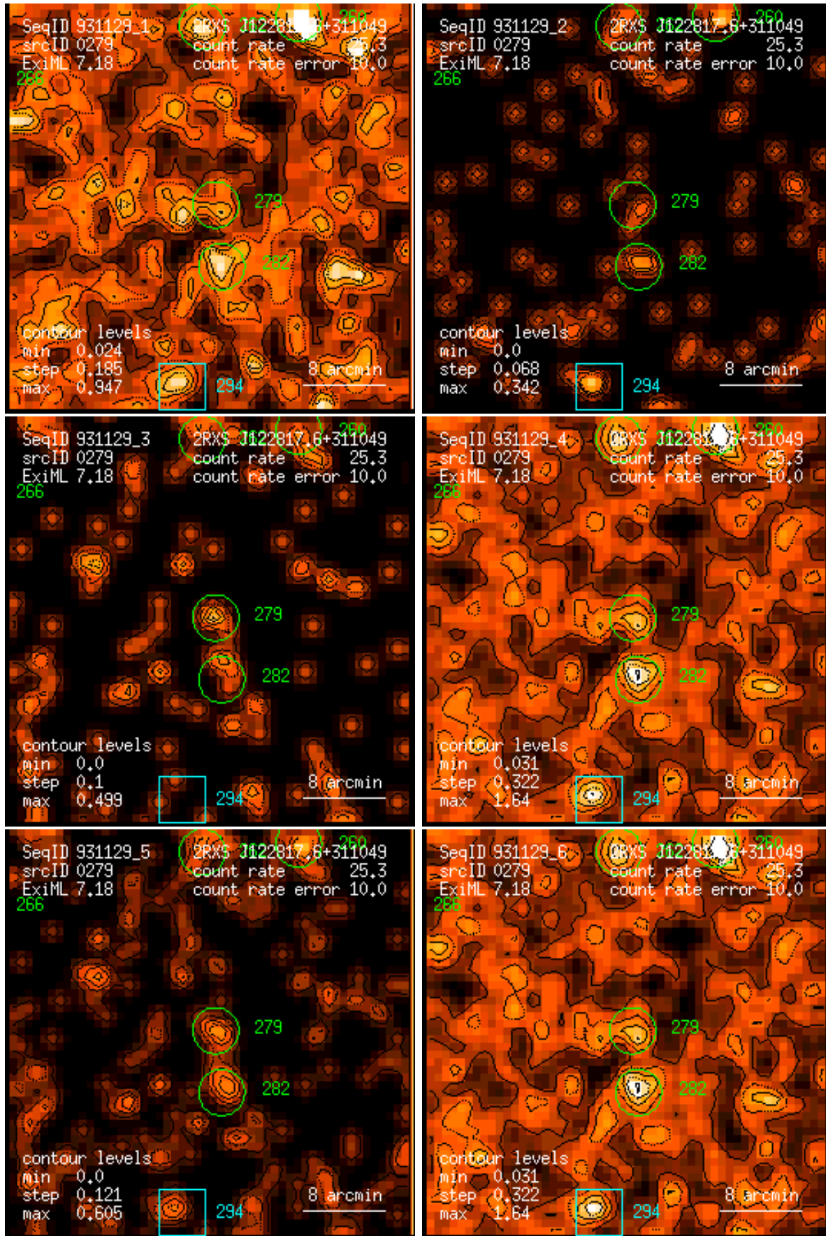
Figure 279: RASS 931129: detection 0279: band rate images, Gaussian filter: (1) PSPC channels 11 – 41, (2) 52 – 90, (3) 91 – 201, (4) 11 – 235, (5) 52 – 201, (6) 11 – 201. Broad band rates in counts/ks. Band rate contour levels in counts/ks/arcmin 2 .
