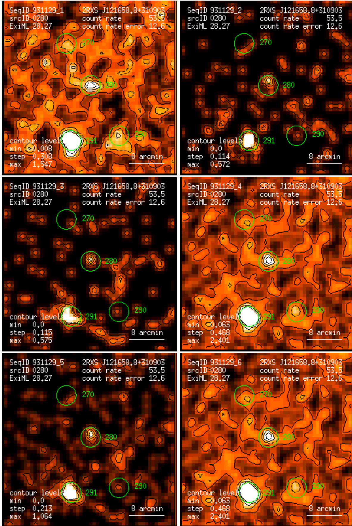
Figure 280: RASS 931129: detection 0280: band rate images, Gaussian filter: (1) PSPC channels 11 – 41, (2) 52 – 90, (3) 91 – 201, (4) 11 – 235, (5) 52 – 201, (6) 11 – 201. Broad band rates in counts/ks. Band rate contour levels in counts/ks/arcmin 2 .
