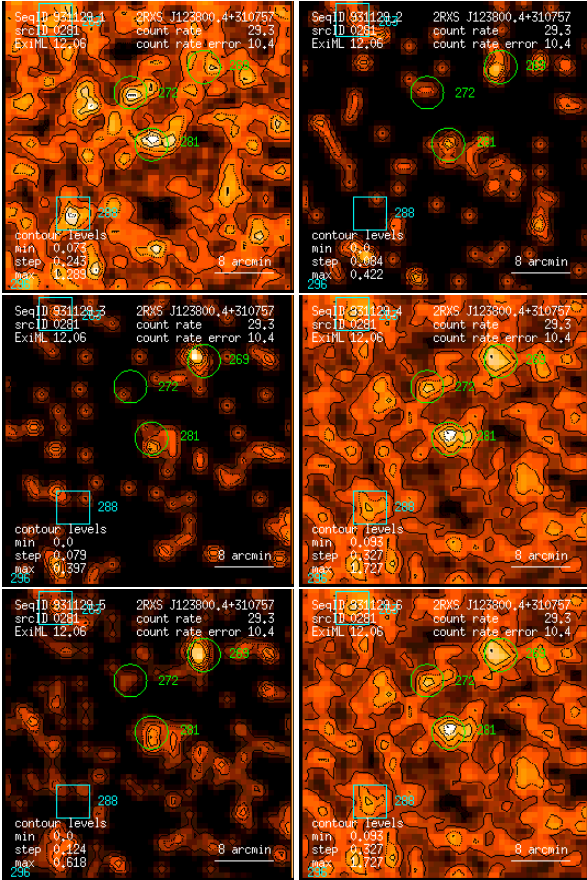
Figure 281: RASS 931129: detection 0281: band rate images, Gaussian filter: (1) PSPC channels 11 – 41, (2) 52 – 90, (3) 91 – 201, (4) 11 – 235, (5) 52 – 201, (6) 11 – 201. Broad band rates in counts/ks. Band rate contour levels in counts/ks/arcmin 2 .
